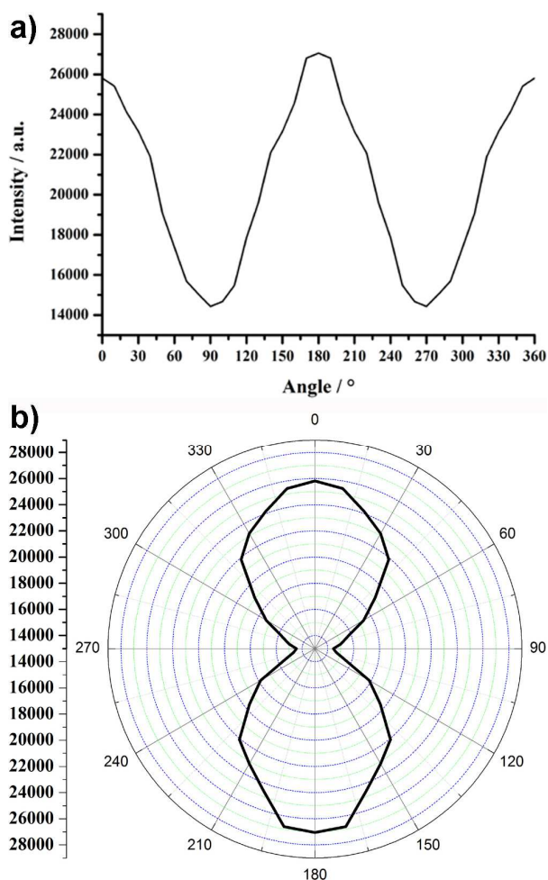
Figure 11. a) Photoluminescence intensity as a function of analyzer angle; b) Polar graph presentation. The excitation wavelength is 340-380 nm and the registration wavelength is 442 nm.
