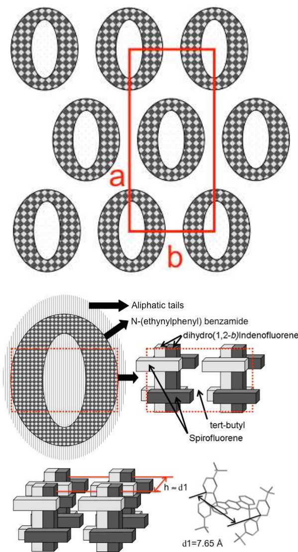
Figure 5. Model of the hollow columns and columnar rectangular phase formed by 1 .
