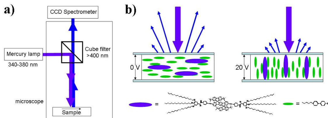
Figure 9. (a) Experimental setup for polarized photoluminescence measurements with compound 1 /5CB mixtures; (b) Schematic representation of the molecular organisation inside the LC cell without and with applied electric field and effect on the emitted blue light.
