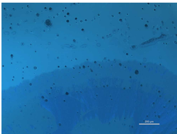
Figure 7. Co-existing isotropic liquid (light-blue) and HT (dark-blue) phases at 195 °C observed upon irradiation at 340 < \lambda_{\text{ex}} < 380 nm (black areas correspond to trapped air bubbles) (same area as in Figure 3a).
