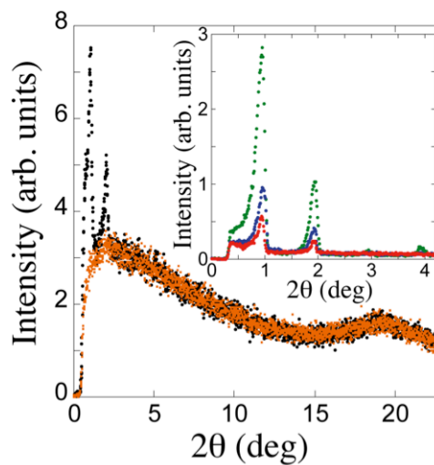
Figure 4. Wide-angle X-ray diffraction patterns for compound BIPH at different temperatures in the phase coexistence range. The intensity is plotted as a function of 2\theta , where \theta is the Bragg angle. Orange points in the diagram are characteristic of a nematic structure (data at 137 °C). Black points in the diagram indicate that a lamellar phase grows within the nematic bulk (data at 135 °C). The inset represents the diffraction patterns obtained with a small-angle goniometer. Red and blue points correspond to the coexistence range as the temperature is lowered. Green points correspond to the low temperature phase (data at 120 °C). All the diagrams were indexed on the basis of a single periodicity.
