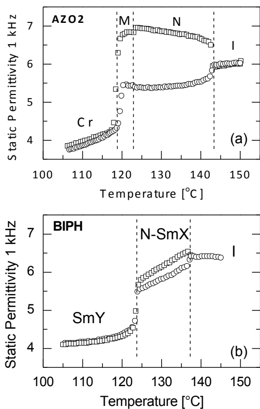
Figure 6. Dielectric permittivity versus temperature for compound AZO2 (top) and compound BIPH (bottom) in cooling runs.
