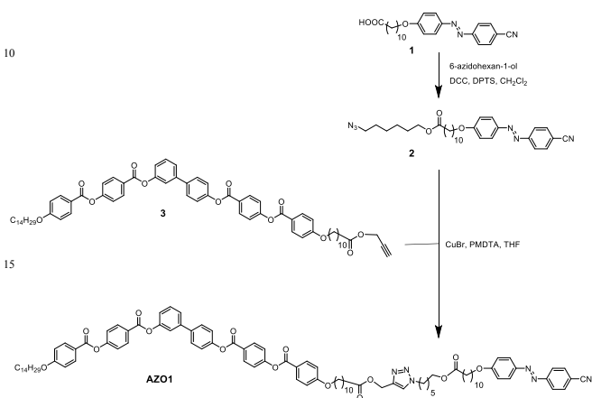
Scheme 2. Synthetic route followed to synthesize dimer AZO1 .
