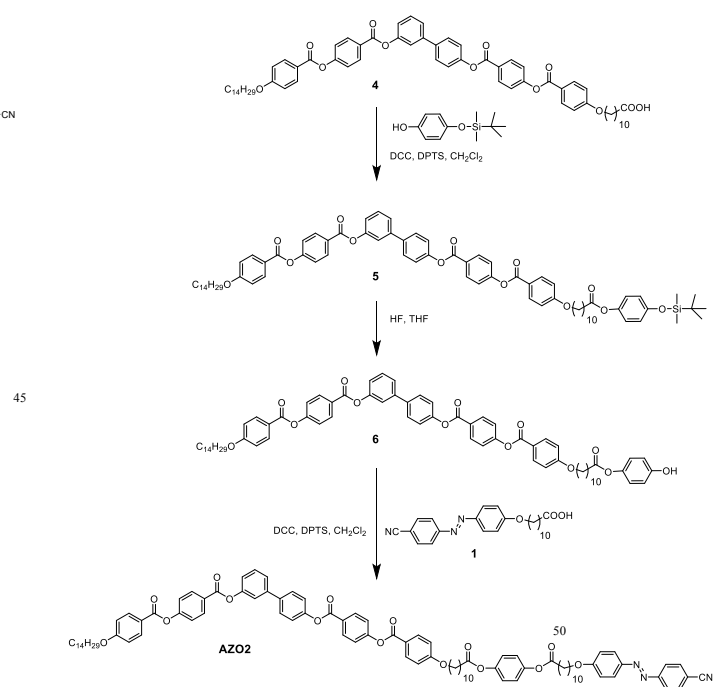
Scheme 3. Synthetic route followed to synthesize dimer AZO2 .
