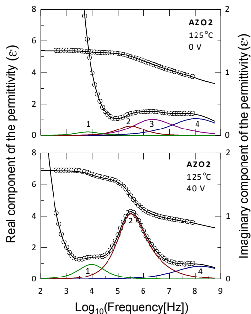
Figure 8. Frequency dependence of the dielectric permittivity of compound AZO2 in the N phase ( T = 125 °C), with no field (top) and with a dc bias field of 40 V (bottom). Black solid lines are fittings according to equation (2) and coloured lines represent the deconvolution into elementary modes.
