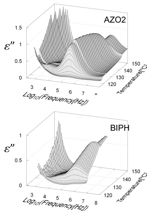
Figure 7. Three-dimensional plot of dielectric losses versus temperature and logarithm of the frequency for compounds AZO2 (top) and BIPH (bottom) under 40 V dc bias field conditions.
