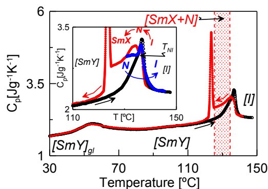
Figure 5. Specific-heat data as a function of temperature for a sample of compound BIPH . Black and red symbols relate to data collected in heating and cooling runs at 1 °C/min, respectively. The inset shows the detail of the specific heat around both the SmX-to-N and the N-to-I phase transitions. Blue symbols correspond to a heating run on slow cooling at 0.5 °C/min from the I phase down to 134 °C. Coexistence regions are marked by shaded areas.
