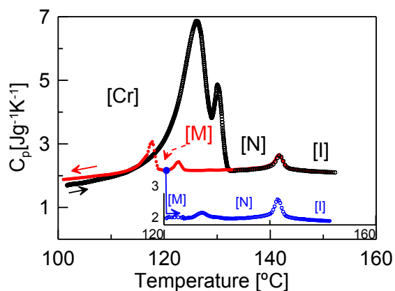
Figure 2. Specific heat capacity data as a function of temperature for a sample of compound AZO2 . Black and red symbols represent data collected on heating and cooling runs at 1 °C/min, respectively. Blue symbols correspond to a heating run from 120 °C after cooling from the isotropic phase without reaching crystallization.
