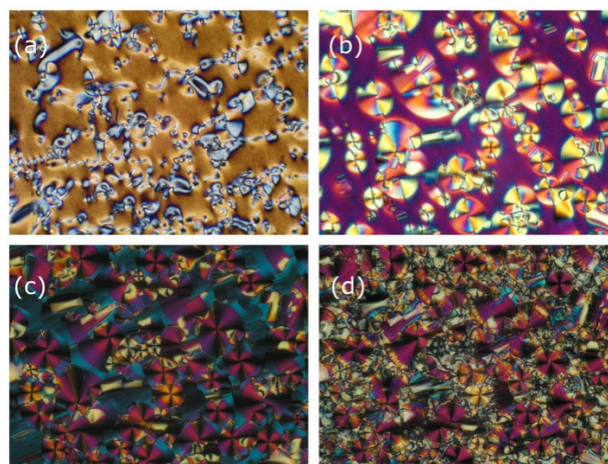
Figure 3. Microphotographs of the textures of compound BIPH : (a) in the N phase at 136 °C, (b) in the N-SmX mesophase at 132 °C, (c) in the SmX at 124 °C, (d) in the SmY phase at 123 °C. The width of the four photographs is about 300 \mu\text{m} .
