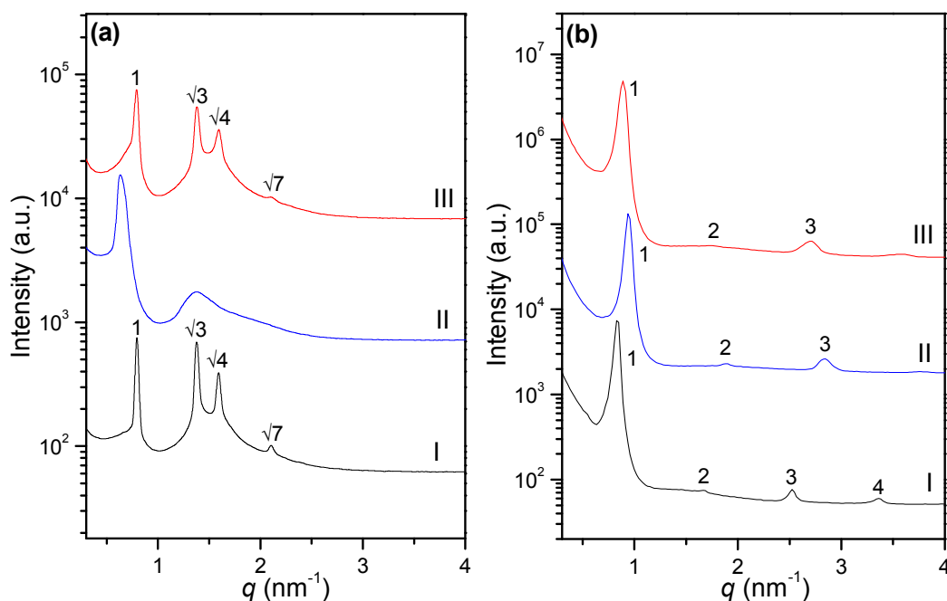
Fig. 9 SAXS patterns for the azo-surfactant/water systems with 50 wt % H 2 O before UV irradiation (I), after UV irradiation (5 min) (II), and followed by visible exposure (5 min) (III) at 25 °C: (a) azo-surfactant A/water; (b) azo-surfactant B/water.
