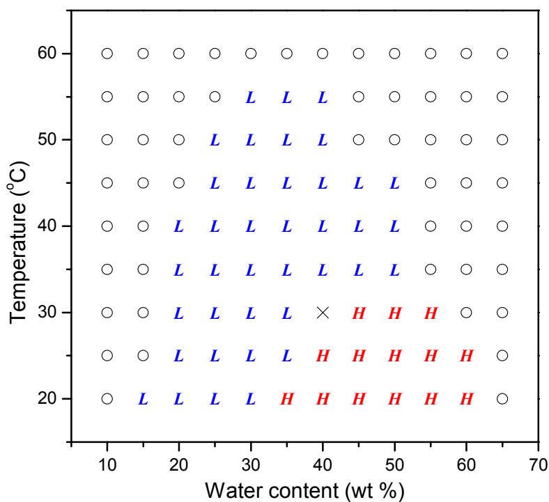
Fig. 5 Data points for the partial phase diagram derived from SAXS patterns of the azo-surfactant A/water binary system. L : Lamellar phase; H : Hexagonal phase; O : Isotropic phase; × : Lamellar and hexagonal.
