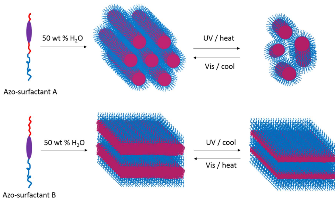
Fig. 10 Schematic illustration of different phase behaviours and stimulus-response properties of azo-surfactants A and B at 50 wt % H 2 O content respectively.
