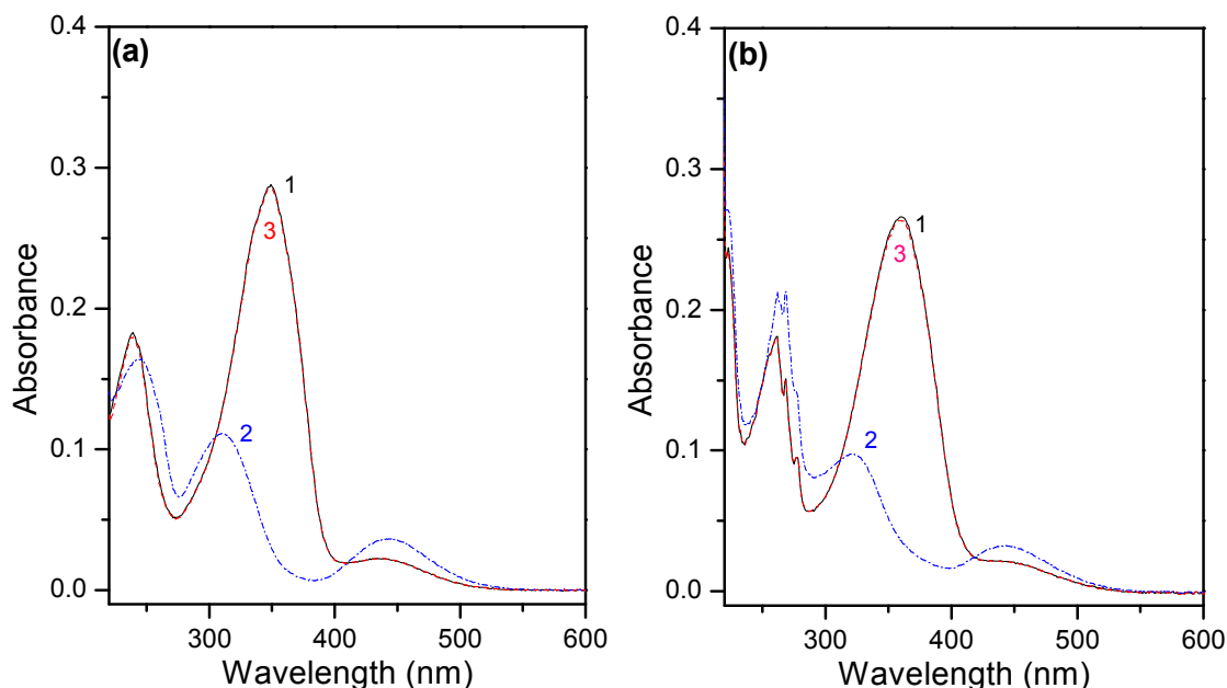
Fig. 8 Influence of photo-irradiation upon absorption spectra of azo-surfactant A (a) and azo-surfactant B (b): (1) before UV irradiation; (2) after UV irradiation (10 min); (3) after UV irradiation followed by visible light exposure (10 min).
