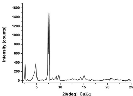
Fig. 5 XRD pattern of an electrodeposited BuPTCDI film.
