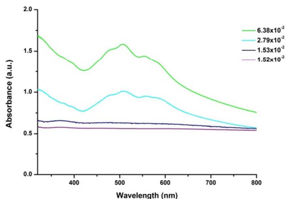
Fig. 7: Absorbance of several different films deposited with differing total charge passed ( C\text{cm}^{-2} , indicated by the inset) showing increased absorbance for the thicker films.
