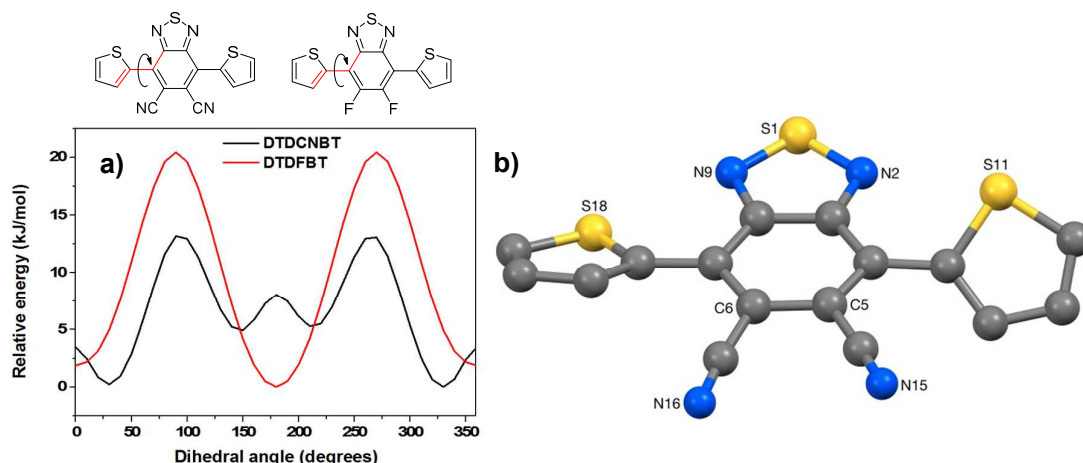
Figure 4: a) Potential energy scan of the T-BT dihedral angle in a DTDCNBT unit (black) and a DFDTBT unit (red) b) Crystal structure of DTDCNBT.
