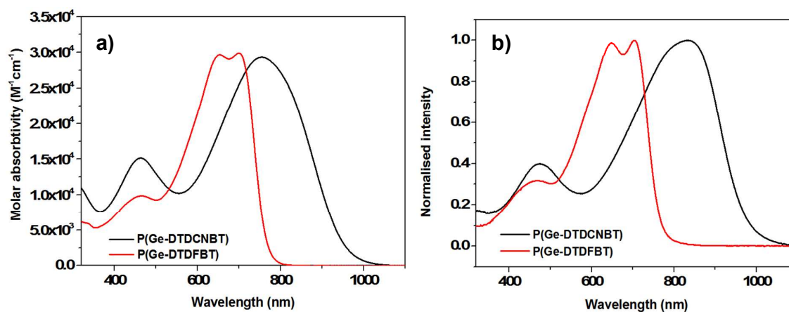
Figure 1: a) Optical absorption spectra of P(Ge-DTDCNBT) and P(Ge-DTDFBT) in chlorobenzene solution ( 16.6 \text{ mg/dm}^3 ) and b) in spun-cast thin film.
