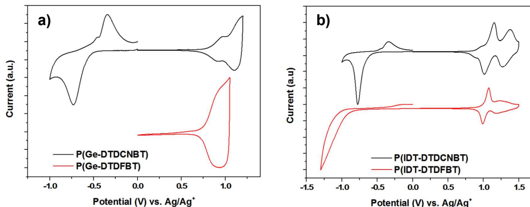
Figure 3: Cyclic voltammograms of thin films of a) P(Ge-DTDCNBT) and P(Ge-DTDFBT) b) P(IDT-DTDCNBT) and P(IDT-DTDFBT) in acetonitrile/ [n\text{-Bu}_4\text{N}]\text{PF}_6 solutions (0.1M) at a scan rate of 100 \text{ mVs}^{-1} )
