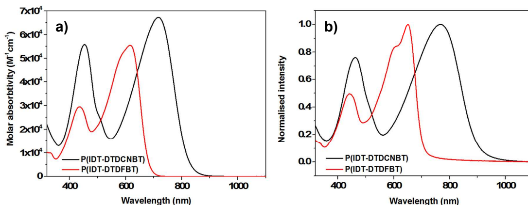
Figure 2: a) Optical absorption spectra of P(IDT-DTDCNBT) and P(IDT-DTDFBT) in chlorobenzene solution (16.6 mg/dm 3 ) and b) in spun-cast thin film.
