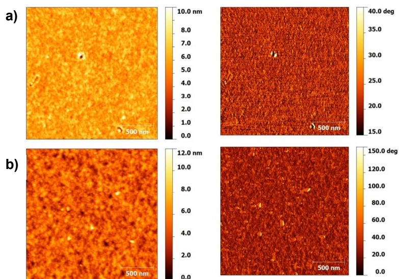
Figure 6: AFM topography (left) and phase (right) of a) P(Ge-DTDCNBT) and b) P(Ge-DTDFBT)
