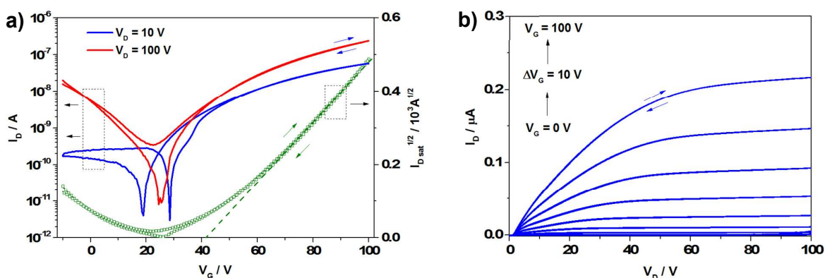
Figure 5: Transfer (left) and output (right) characteristics of P(Ge-DCNDTBT), under positive voltages in the TG/BC device configuration.
