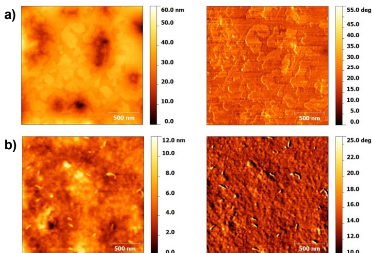
Figure 7: AFM topography (left) and phase (right) of a) P(IDT-DTDCNBT) and b) P(IDT-DTDFBT)
