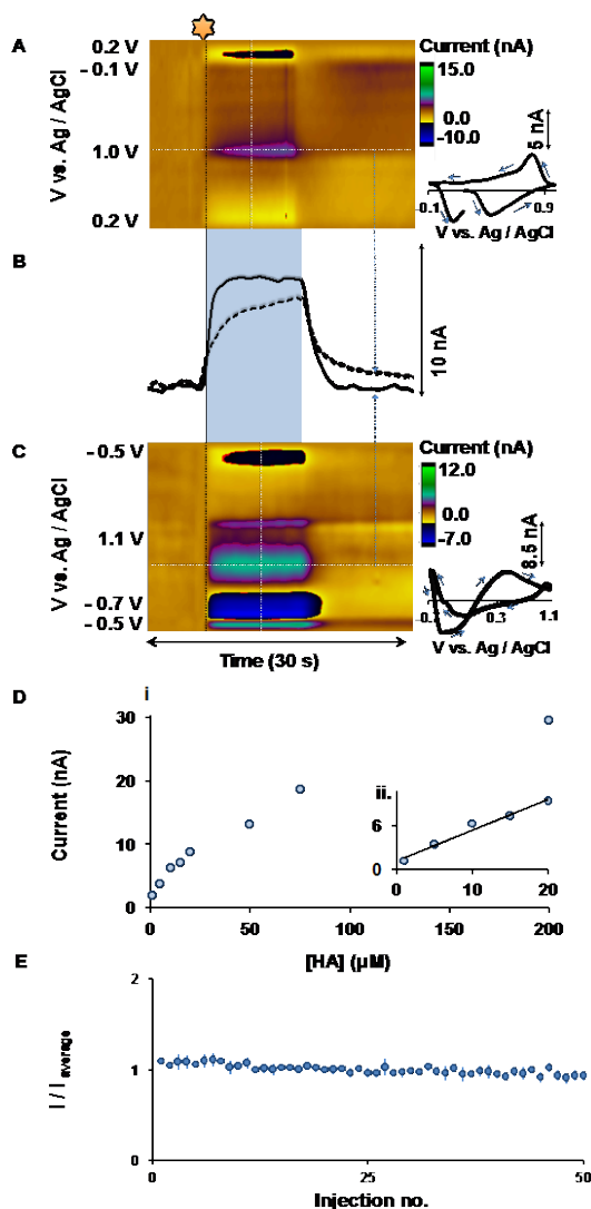
Figure 3: A & C show color plots for FIA of 20 μM histamine with the serotonin and HSW waveforms respectively. CVs extracted from vertical dashed lines are shown on the right. B shows Current vs. time traces from the horizontal dashed lines from color plots. D shows (i) Calibration curve, (ii) Linear dynamic range ( n=4 \pm \text{SEM} ). E Stability of CFM over 50 consecutive injections of 10 μM histamine ( n=4 \pm \text{SEM} ).
