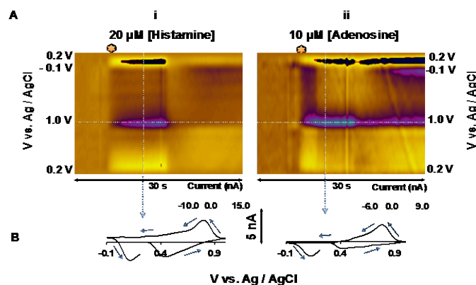
Figure 1: A shows color plots for FIA of (i) 20 \mu\text{M} histamine (ii) 10 \mu\text{M} adenosine. B shows CVs extracted from the vertical dashed lines from (i) and (ii).
