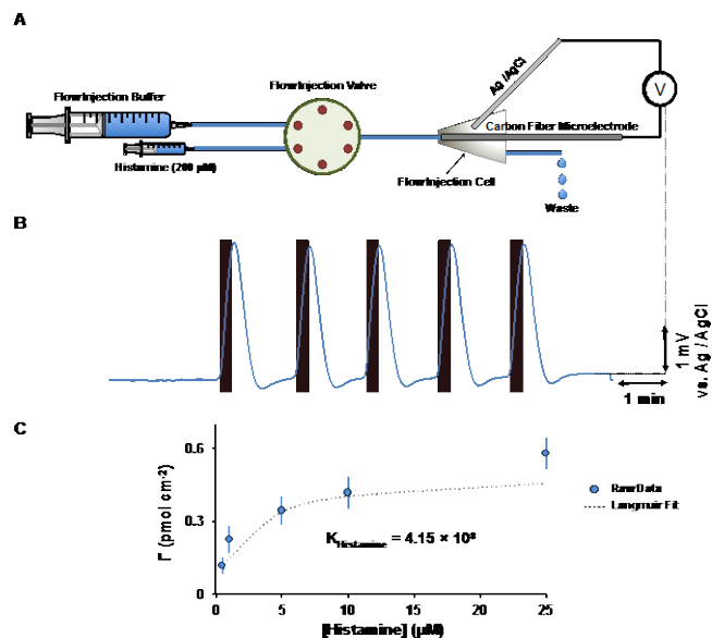
Figure 2: A shows the schematic diagram of the experimental setup used for potentiometric experiments. B shows the experimental potentiometric data for five consecutive injections of histamine (200 \mu\text{M} ) on CFM. C Langmuir isotherm for histamine adsorption on CFMs in Tris buffer.
