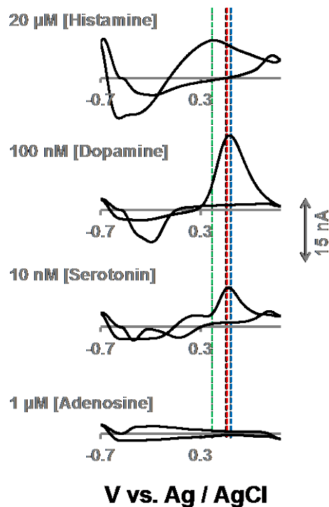
Figure 4: CVs for 20 μM histamine, 100 nM dopamine, 10 nM serotonin and 1 μM adenosine with in vitro FIA using HSW on CFMs. Vertical dashed lines indicate potential positions of peaks.
