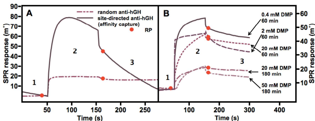
Figure 2. SPR responses to 600 nM hGH by sensor surfaces prepared by different anti-hGH immobilization techniques. A – Anti-hGH immobilized in a random (---) and site-directed (—) manner. B – Protein G mediated anti-hGH immobilization after different DMP cross-linking procedures. 1 – Baseline phase, 2 – association phase, 3 – dissociation phase, RP – report points.
