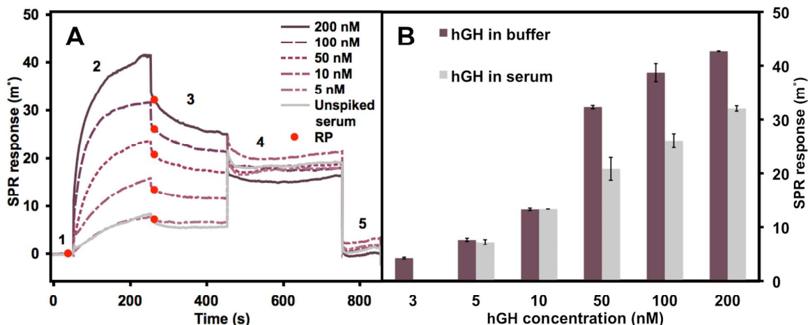
Figure 6. The responses of the developed SPR immunosensor to a range of hGH concentrations in human serum samples (A) and comparison of SPR immunosensor responses to hGH in PBS and human serum samples (B).
