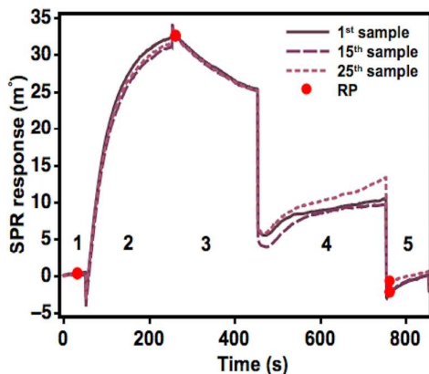
Figure 4. The responses of the developed SPR immunosensor to 50 nM hGH samples upon repeated measurements.
