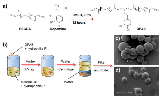
Figure 1 - Formation of the dopamine containing poly( \beta -amino ester)(DPAE) via Michael type addition (a). This DPAE pre-polymer could then be emulsified in oil and photocrosslinked into beads ready for filtration and collection (b). SEM images show spherical beads formed from PEG (c) or DPAE (d).
