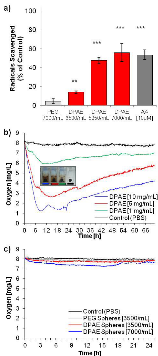
Figure 3 - DPAE scavenges radicals and reduces dissolved oxygen content in PBS. Microspheres scavenge the DPPH stable radical (a) in a dose dependent manner up to a level scavenged by 10 μM ascorbic acid (n=4, error bars represent +/- standard deviation, two-tailed Student's t-test marking difference to PEG spheres with p-value < 0.001 (***) and p-value < 0.01 (**)) Bulk preparations of the DPAE reduced the dissolved oxygen content of PBS (b) which results in a darkening of the DPAE due to oxidation of the catechol group after two days (images of cuvettes - insert). Microspheres of DPAE, at the same concentrations as used for the radical scavenging assay and toxicity assays, showed only a slight decrease in dissolved oxygen content (c).
