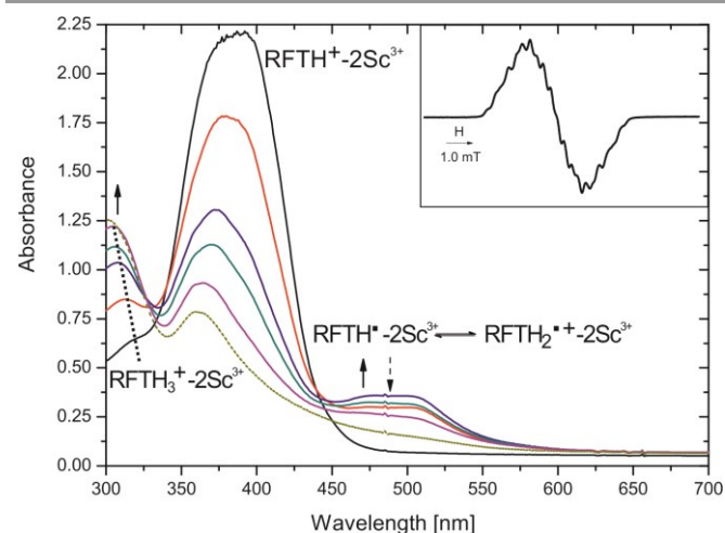
Figure 2. UV-vis absorption spectra of ethylbenzene (5.8 mM) and RFT (0.14 mM) in the presence of \text{Sc}(\text{OTf})_3 (0.68 mM) and HCl (2.7 mM) during irradiation with blue light in deaerated MeCN at 298 K under nitrogen (straight: 0 s, 60 s, 120 s, 180 s, 360 s; dashed: 2h). Inset: ESR-spectrum of ^2\text{RFTH}_2^{\bullet+} \cdot 2\text{Sc}^{3+} generated in the photocatalytic reaction RFT (3.0 mM) with ethylbenzene (20 mM), \text{Sc}(\text{OTf})_3 (10 mM) and 10 mM HClO 4 in deaerated MeCN at 298 K. Parameters obtained by computer simulation: g = 2.0033 , a(\text{N}^5) = 6.7 G, a(\text{N}^{10}) = 4.6 G, a(\text{H}^5) = 10.6 G, a(3\text{H}^8) = 2.9 G, a(\text{N}^{10}\text{-CH}_2) = 4.3 G; see the ESI for the labelling scheme.
