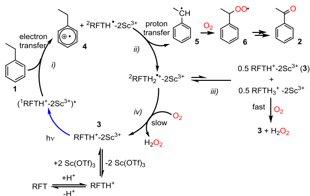
Scheme 3. Proposed mechanism for the photocatalytic aerobic oxidation of ethylbenzene ( 1 ) to acetophenone ( 2 ) with RFT in presence of Sc 3+ -ions and HCl.
