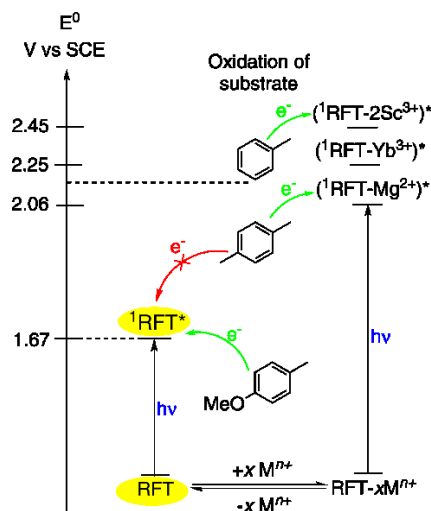
Figure 1. Enhanced reduction potentials E^{\circ}({}^1\text{RFT}^*/{}^2\text{RFT}^-) of RFT-metal ion complexes (RFT- x\text{M}^{n+} ). 8,9
