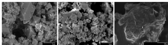
Fig. 4. SEM micrographs of the ECM heated to 515°C in air, showing nano and micron sized diamonds. The left hand panel shows diamond crystal which are growing on a carbon substrate.
