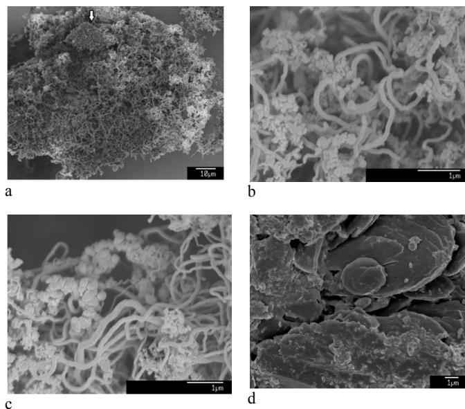
Fig. 1. (a) and (b) show SEM morphology of the as-synthesised ECM. It contains a mixture of CNTs and carbon nanoparticles, and some micrometer-sized carbon particles such as one pointed by arrow in (a). (c) and (d) show SEM morphology of the material after heated to 400 and 570°C, respectively, and subsequently cooled down to the room temperature under ambient air flow of 100 mL \text{min}^{-1} (see Fig. 3b-upper panel).
