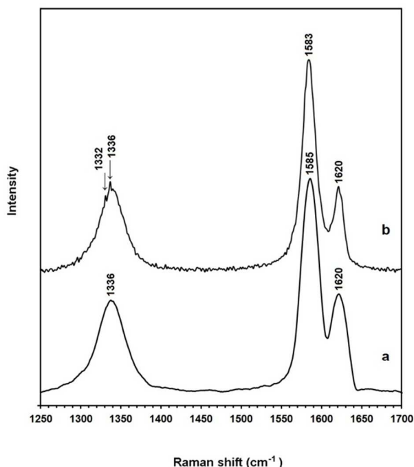
Fig. 7 Raman spectra of (a) the as-synthesised ECM and (b) the ECM heated in air to 515 °C (see Fig. 3-down panel) showing the peak of diamond at 1332 cm -1 .
