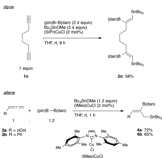
Scheme 2 Borylstannylation of a diyne and allenes.
