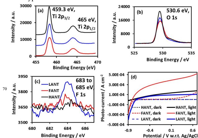
Fig. 3. (a), (b), and (c) represent XPS spectra for Ti 2p, O 1s, and F 1s, respectively, and (d) shows the plots of photocurrent versus potential under dark and under AM 1.5G simulated sunlight, for the three types of nanotubes.
