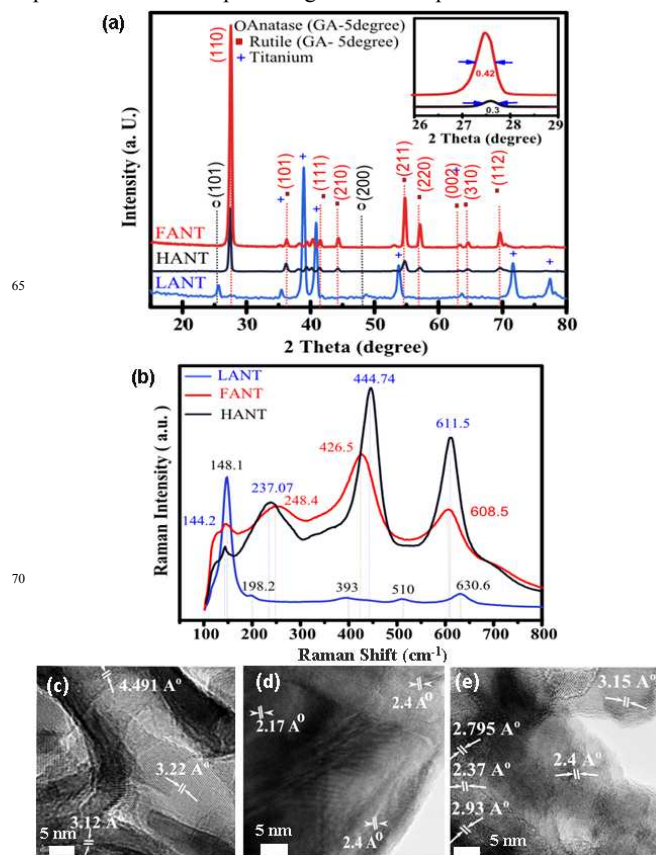
Fig. 2. (a) Peak-indexed GIXRD patterns of LANTs (blue), HANTs (black) and FANTs (red) while the inset is a comparative illustration of the full peak widths at half of maximum intensities of FANTs and HANTs; (b) Raman spectra of LANTs (blue), HANTs (black) and FANTs (red); (c), (d) and (e) TEM lattice images of LANTs, HANTs and FANTs, respectively.
