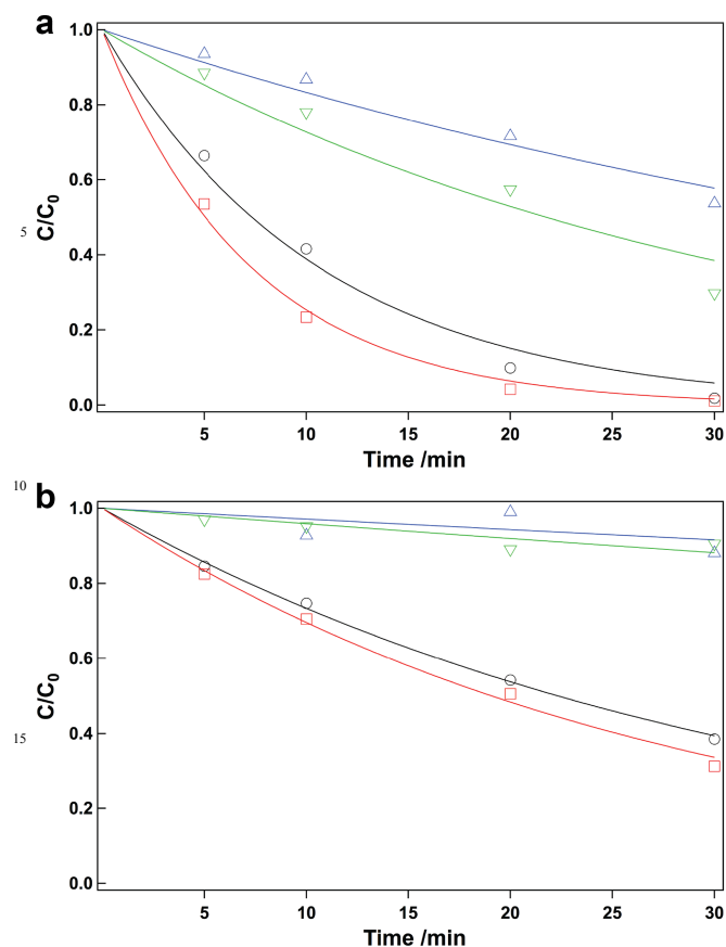
Figure 2. Photocatalytically induced dye degradation in coacervate micro-droplets. Plots show the time-dependent reduction in the normalized dye concentration sequestered into (a) TiO 2 NS/PDDA/KPSE and (b) TiO 2 NS/PDDA/ATP; for MB (black line and circles), MB after the addition of 5 M NaCl (red line and squares), SRhB (blue line and triangles) and SRhB after the addition of 5 M NaCl (green line and inverted triangles).
