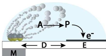
Fig.1 Microengine-assisted mixing for electrochemical measurements. Schematic illustration of microengine-enhanced bubbles flow. A: OP Nerve Agents; P: p -nitrophenol; E: Working Electrode; D: Distance between Working Electrode to Mg-Microengines (5 mm); M: Magnet.
