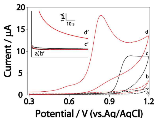
Fig.4 Cyclic Voltammograms of (a) 0.1 M KCl solution without microengines, (b) 0.1 M KCl solution with microengines, (c) 20 mM paraoxon in 0.1M KCl without microengines and (d) 20 mM paraoxon in 0.1M KCl with microengines. Inset: Amperograms of (a') 0.1 M KCl solution without microengines, (b') 0.1 M KCl solution with microengines, (c') 20 mM paraoxon in 0.1M KCl without microengines and (d') 20 mM paraoxon in 0.1M KCl with microengines
