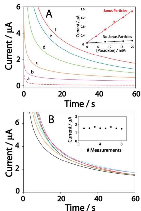
Fig.5 A) Amperograms obtained in the presence of microengines for different paraoxon concentrations (a) 0, (b) 4, (c) 8, (d) 12, (e) 16 and (f) 20 mM in 0.1M KCl. Inset: Calibration plot comparison toward paraoxon obtained without (square) and with (circle) microengines, current sampled at 60 sec (n=3); B) Reproducibility of the response for 20 mM paraoxon solution in KCl 0.1 M in presence of microengines (n=8). Applied potential, 0.9 V (vs. Ag/AgCl).
