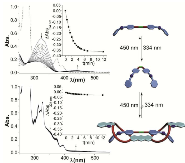
Figure 3 E \rightarrow Z photoisomerisation of E-1 (40 \mu\text{M} in \text{CHCl}_3 : \text{CH}_3\text{CN} = 2 : 1 ) upon irradiation with 334 nm in the absence (top) and presence (bottom) of an equimolar amount of host 3 (dashed line shows spectrum of pure 3 ).
