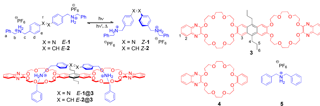
Figure 1 Isomerization of divalent azobenzene and stilbene axles 1 and 2 , divalent host 3 , monovalent reference compounds 4 and 5 , as well as divalent pseudo[2]rotaxanes E-1@3 and E-2@3 .
