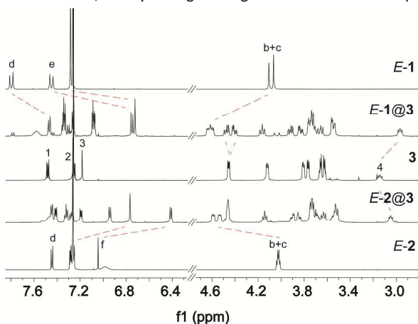
Figure 2 1 H NMR experiment of the complexation of azobenzene axle E-1 (top) as well as E-2 (bottom) to host 3 (500 MHz, \text{CDCl}_3 : \text{CD}_3\text{CN} 2 : 1 , 1.4 mM). The dotted lines indicate the shifting of selected protons upon formation of the complex.
