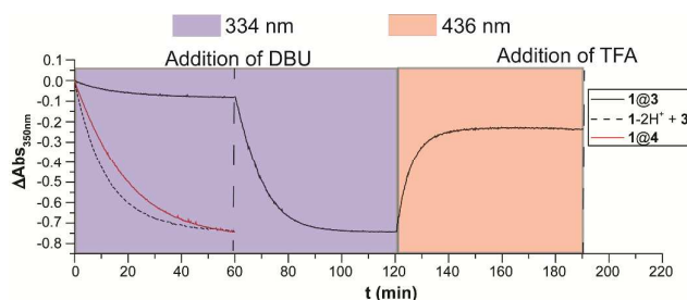
Figure 4 E \rightarrow Z photoisomerisation of E-1 in presence of 3 ( 1@3 , solid black line), deprotonated E-1 in presence of 3 ( 1-2H^+ + 3 , dashed black line), and E-1 in presence of 4 ( 1@4_2 , solid red line) monitoring azobenzene absorption maximum at 350 nm upon irradiation at 334 nm ( 40 \mu M in CHCl_3 : CH_3CN = 2 : 1 ). After 60 min DBU (4 equiv.) was added to the solution of E-1@3 leading to deprotonation and recovery of photoreactivity. Subsequent Z \rightarrow E photoisomerisation at 436 nm and addition of TFA (4.1 equiv.) reprotonates the axle and resets the system. Note that the system does not recover fully because of the photostationary state of deprotonated 1 and photochemical side reactions of 3 .
