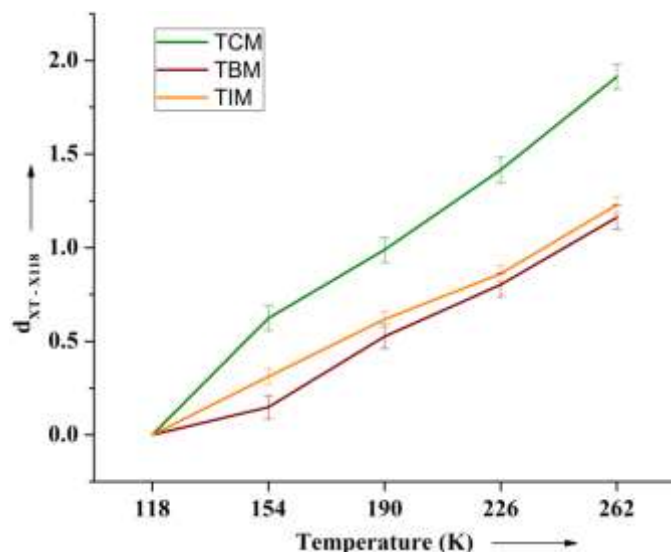
Fig. 5 Plot of the change in average interhalogen interaction distance vs. temperature.
