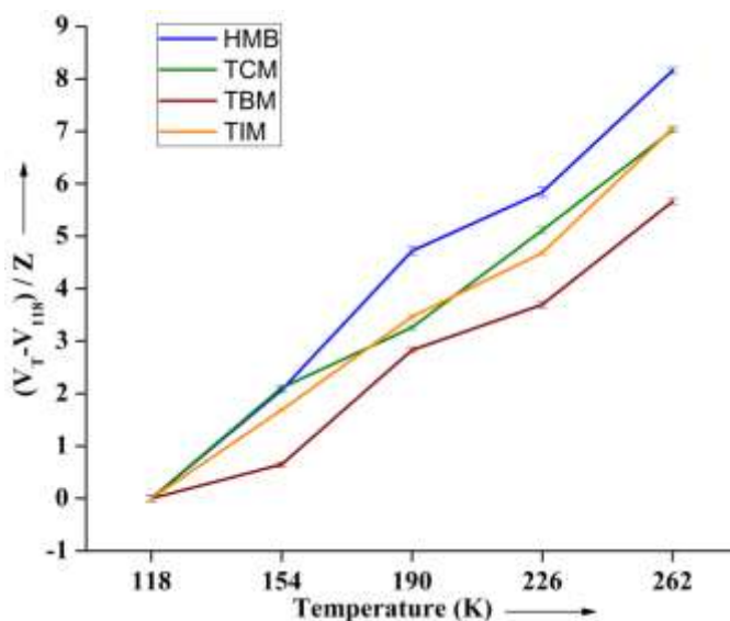
Fig. 2 Plot of the change in unit cell volume/ Z vs. temperature.
