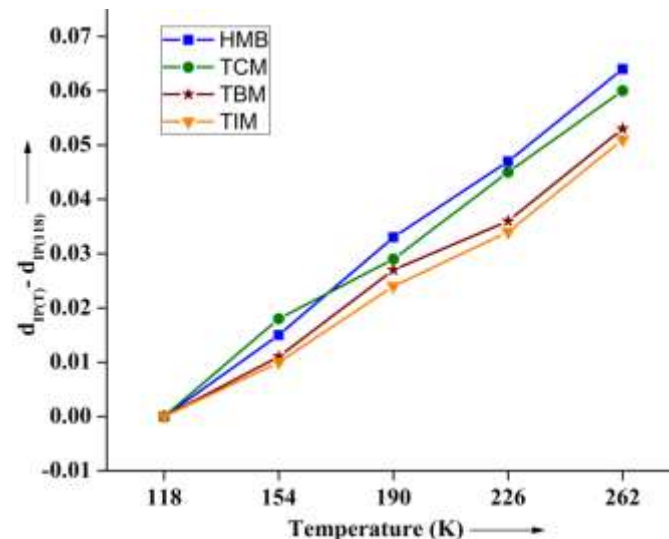
Fig. 3 Plot of change in interplanar distance vs. temperature.
