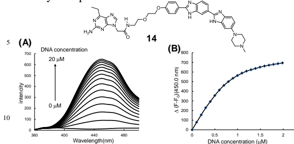
Fig. 6. (A) Changes in fluorescence spectra of 14 (0.1 \mu\text{M} ) in 50 mM MES (pH 7.0), 100 mM NaCl with increasing duplex DNA (AP0bp) concentration. (B) Changes in fluorescence intensity at 450 nm are plotted versus the DNA concentration.
