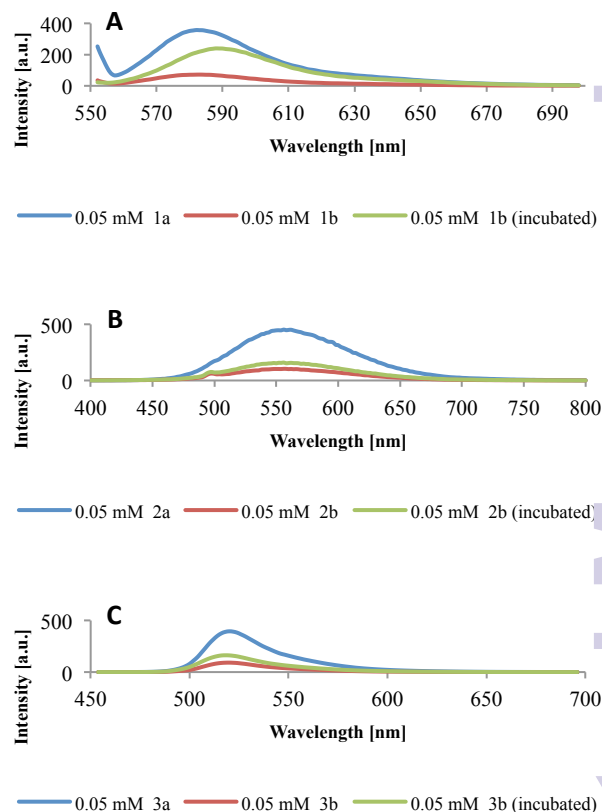
Figure 4: Fluorescence spectra. A) 1a , 1b and 1b (incubated) in Britton-Robinson buffer (10 mM, pH 5.0). B) 2a , 2b and 2b (incubated) in TRIS-HCl buffer (10 mM, pH 7.4). C) 3a , 3b and 3b (incubated) in TRIS-HCl buffer (10 mM, pH 7.4).
