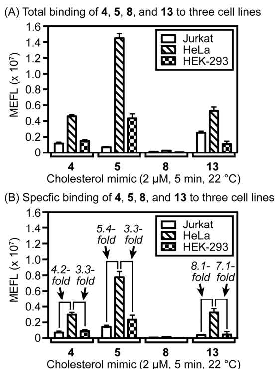
Fig. 3. Total binding (A) and specific binding (B) of compounds 4 , 5 , 8 , and 13 to three mammalian cell lines. Cells in media containing 10% serum were treated with compounds, without (A) and with (B) excess ezetimibe ( 3 , 200 \mu\text{M} ), in triplicate at 22 ^{\circ}\text{C} for 5 min. Jurkat, HeLa, and HEK-293 cells were suspended in media prior to treatment and analysis of fluorescence by flow cytometry.
