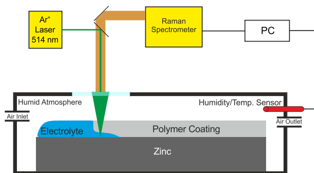
Fig. 1 Schematic view of setup used for the experiments.
