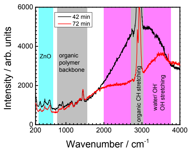
Fig. 2 Example in situ Raman spectra after two different delamination times as indicated on the graph. Regions with contributions from the different species in the system are labelled.
