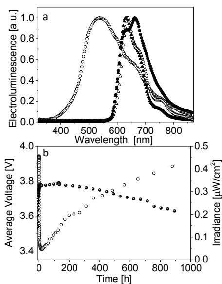
Figure 3. (a) Normalized EL spectra obtained at 10 V of devices with BODIPY (open circles) and Zn-porphyrin (close circles) references, as well as 1 (open triangles) and 2 (close triangles) devices. (b) Average voltage (open symbols) and irradiance (full symbols) vs time of 1 device driven by a pulsed current using a block wave at a frequency of 1 kHz with a duty cycle of 50% and an average current of 10 mA.
