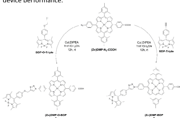
Scheme 1. Synthesis of BODIPY-porphyrin dyads 1 and 2.
