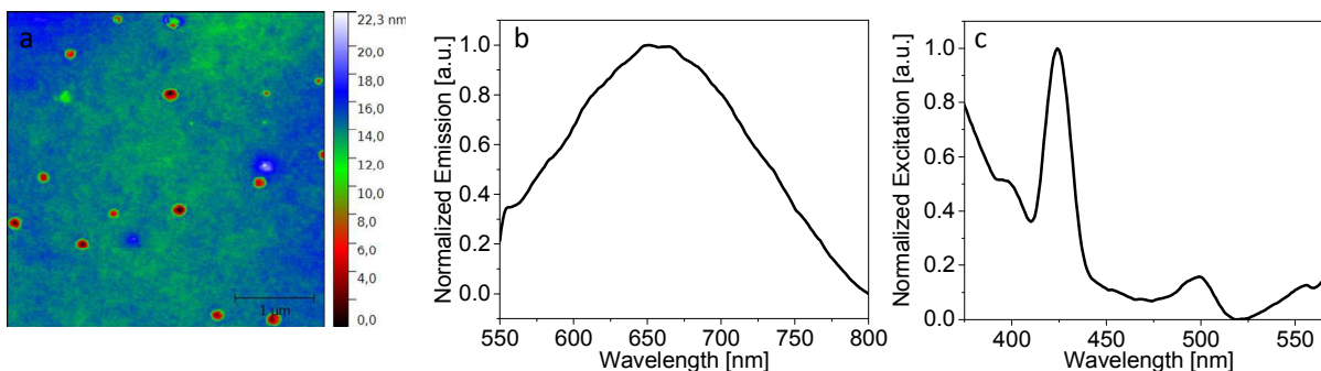
Figure 2. (a) AFM images of 1 films with a thickness of 110 nm. (b) Emission spectra of 1 films upon excitation at 490 nm. (c) Excitation spectra of 1 films when monitoring the emission at 660 nm.
