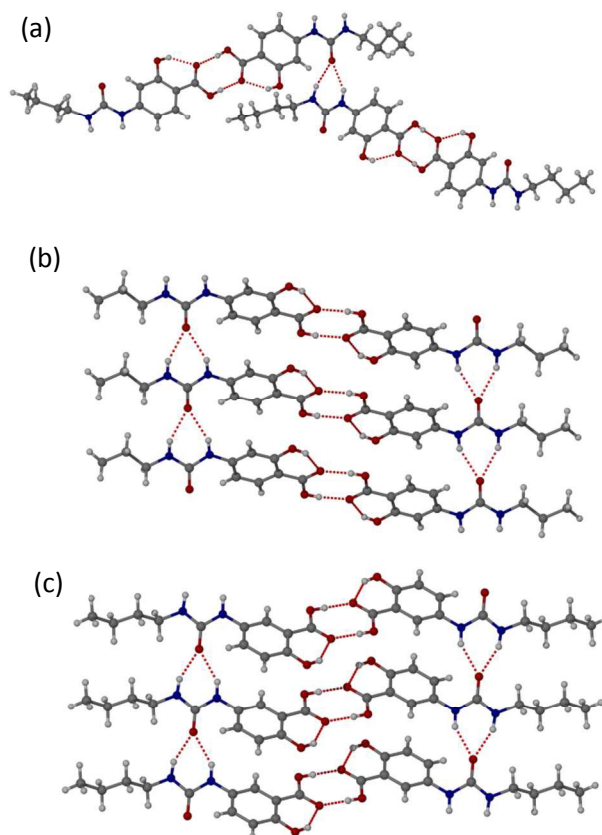
Figure 3. (a) Twisted 2D urea hydrogen bonding in 1a ; (b) parallel packing in 1c with relatively long \text{NH}\cdots\text{O} interactions; (c) short \text{NH}\cdots\text{O} interactions in the gelator 2a . Selected hydrogen bonding distances (Å) for compound 1a : Acid dimer \text{O}\cdots\text{O} 2.606(2), 2.634(2); urea tape \text{N}\cdots\text{O} 2.986(3), 2.880(2), 2.814(2) and 3.072(2), compound 1c , \text{O}\cdots\text{O} 2.892(3), \text{N}\cdots\text{O} 2.911(3), 2.892(3); compound 2a , \text{O}\cdots\text{O} 2.629(6); \text{N}\cdots\text{O} 2.797(7), 2.816(7).
