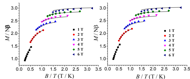
Fig. 2 Reduced magnetization data for 1 (left) and 2 (right). The solid lines represent the best fit to the data.
