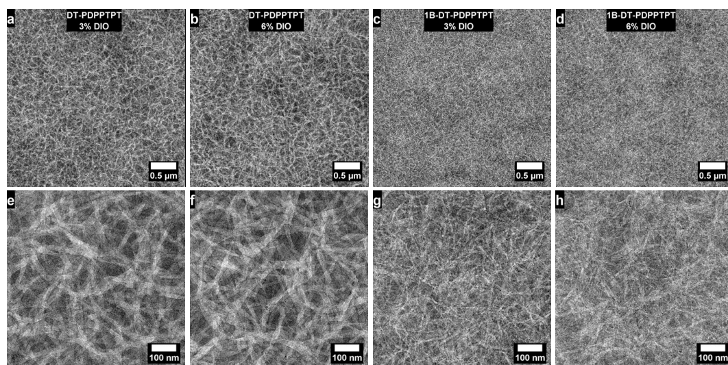
Fig. 3. TEM images of the active layers of DT-PDPPTPT processed with 3% DIO (a, e), DT-PDPPTPT with 6% DIO (b, f), 1B-DT-PDPPTPT with 3% DIO (c, g) and 1B-DT-PDPPTPT with 6% DIO (d, h).
