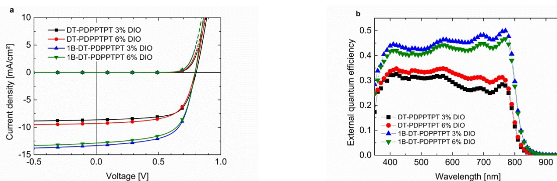
Fig. 2. (a) Current density – voltage ( J - V ) and (b) external quantum efficiency (EQE) of DT-PDPPTPT:[70]PCBM and 1B-DT-PDPPTPT:[70]PCBM solar cells processed from chloroform using 3% and 6% of DIO as co-solvent.
