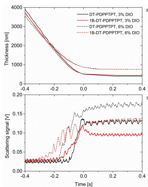
Fig. 4. Drying curve (a) and scattering signal of laser light (b) on the mixture of polymer, fullerene, solvent and co-solvent during spin coating versus time. The signals of different experiments are manually synchronized at the point of drying for the chloroform.
