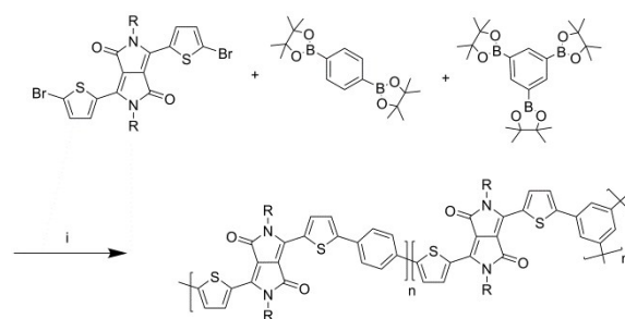
Scheme 1 Polymerization of branched DT-PDPPTPT, using a trifunctional phenylene core as branching unit. R = 2-decyltetradecyl, (i) Pd 2 dba 3 , PPh 3 , K 3 PO 4 , toluene/H 2 C 115°C. m/(m+n) = 0, 0.01, \text{ or } 0.05 .
