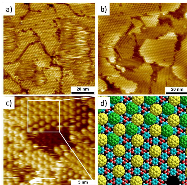
Fig. 2 Epitaxial growth of the 2nd fullerene layer. (a), (b) STM appearances of the multilayer growth imaged with unstable and stable tips, respectively. A representative high resolution STM image (c) and a tentative molecular model (d) of an area with empty COF-1, host-guest assembly C_{60} @COF-1 and assembly with two layers of fullerene. Fullerenes of the first and the second layers are colored yellow and green respectively. (a, b, c) V_{\text{bias}} = -0.900 V, I_{\text{set}} = 0.02 nA.
