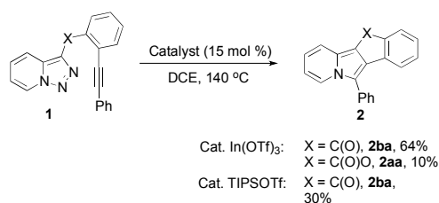
Scheme 3 Lewis acid - catalyzed transannulation reaction of pyridotriazoles.
