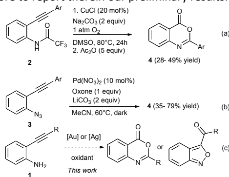
Scheme 1 [M]-catalyzed synthesis of 4 H -benzo[d][1,3]oxazin-4-ones
