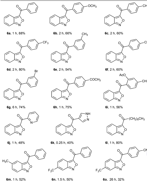
Scheme 4 [Ag]-catalyzed oxidative cyclization – Substrate scope
