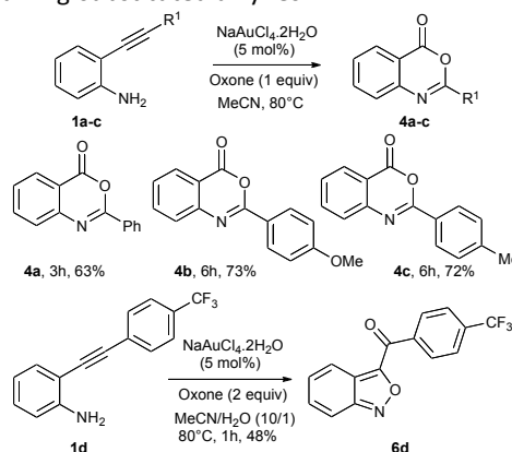
Scheme 2 [Au]-catalyzed oxidative cyclization
