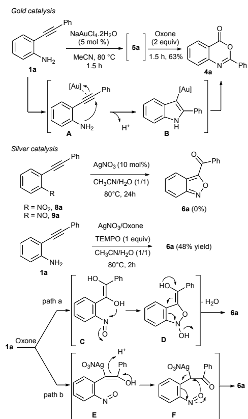
Scheme 3 [Ag]- and [Au]-mechanistic investigations and proposed mechanisms
