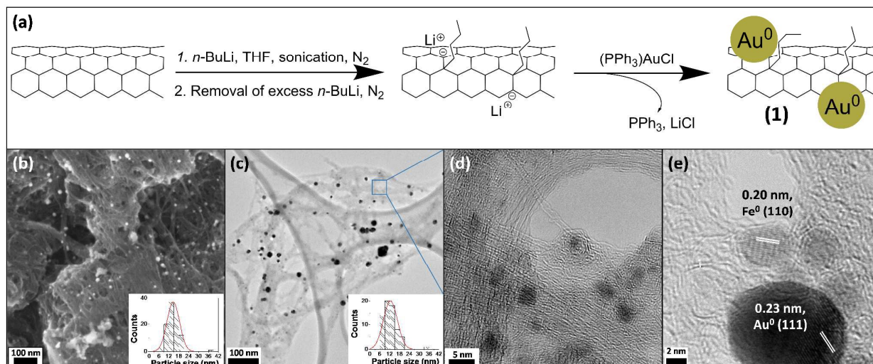
Fig. 1 (a) Scheme showing the generation of [(n\text{Bu-SWCNT})^{\ominus}\cdot\text{Li}^{\oplus}] and proposed formation of AuNPs following \text{ClAu}(\text{PPh}_3) addition to afford n\text{Bu-SWCNTs}/\text{AuNPs} , ( 1 ). Electron microscopy characterisation of ( 1 ): (b) SEM characterisation. Inset shows the particle size distribution of AuNPs. (c) Low resolution TEM image showing AuNPs supported on SWCNT bundles (note the presence of a holey amorphous carbon film support). Inset shows the particle size distribution of AuNPs. (d) HRTEM image of the selected region in Fig. c (blue box) showing the presence of SWCNT bundles and individualized SWCNTs. (e) High magnification HR-TEM image showing two NPs with lattice spacing consistent with \text{Au}^0 and \text{Fe}^0 . Iron catalyst nanoparticles are present, remaining from the HiPco SWCNT synthesis.
