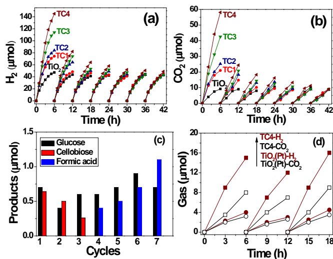
Fig. 3 Time profiles of (a) H 2 production and (b) CO 2 production from the suspension of TiO 2 (Pt) and cellulose immobilized TiO 2 (Pt) samples on repeated cycling. (c) HPLC analysis results on the production of cellobiose, glucose and formic acid from the TC4 sample during repeated cycles. (d) H 2 and CO 2 production from natural sunlight irradiation.
