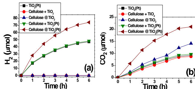
Fig. 2 Time profiles of (a) \text{H}_2 production and (b) \text{CO}_2 production from the suspension of \text{TiO}_2(\text{Pt}) , mixed cellulose with \text{TiO}_2 and \text{TiO}_2(\text{Pt}) , and cellulose immobilized \text{TiO}_2 and \text{TiO}_2(\text{Pt}) samples. Reaction conditions: 15 mg samples suspended in 50 ml de-aerated aqueous solution, UV-Visible light irradiation (iron-halide lamp), reaction temperature (293 K ~ 313 K).
