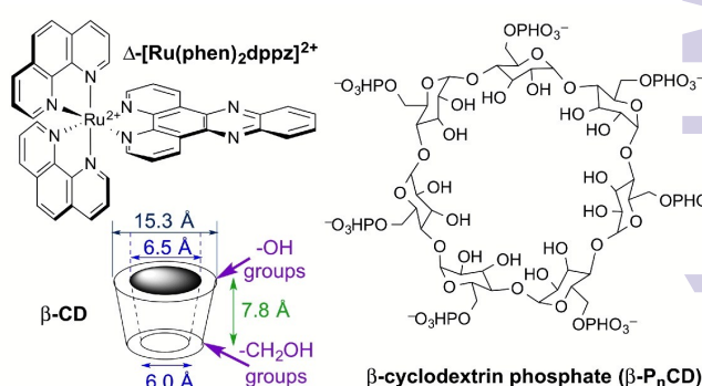
Fig 1 Representative structures for this study.
