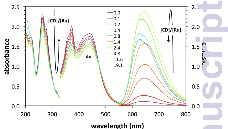
Fig 2 Absorption and emission spectra of \Delta -[Ru(phen) 2 dppz] 2+ with added \beta -CD-phosphate. \lambda_{\text{ex}} = 410 \text{ nm} ; [\text{Ru}] = 20 \mu\text{M} . Legend shows [\beta\text{-P}_n\text{CD}]/[\text{Ru}] ratios.
