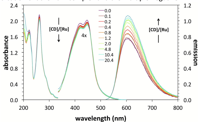
Fig 3 Absorption and emission spectra of \Delta -[Ru(phen) 3 ] 2+ with added \beta -CD-phosphate. \lambda_{\text{ex}} = 470 nm; [Ru] = 20 \mu M; legend shows [\beta\text{-P}_n\text{CD}]/[\text{Ru}] ratios.
