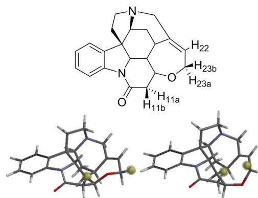
Fig. 3 Strychnine with key protons labelled (above) with major (~98%, lower left) and minor (~2%, lower right) conformers with H11b and H23b highlighted for clarity.
