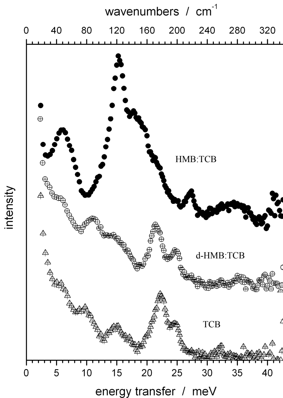
Figure 2 (neutron data)
