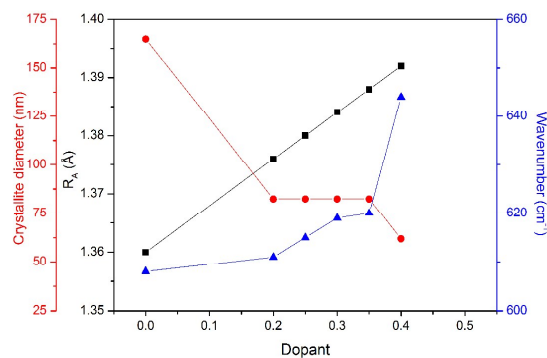
Fig. 7 – The relationship between the average radii of A-site cations ( R_A ), crystallite diameter and wavenumber for the range of doped LSMO materials. Black squares correspond to R_A , red circles to the crystallite diameter, and blue triangles to the Mn-O wavenumber. Connecting lines are included as a guide to the eye.
