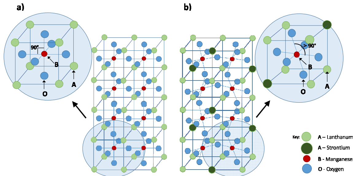
Fig. 1 - Structure of perovskites of the type ABO_3 . Figure 1a shows the undoped parent compound LaMnO_3 and Figure 1b shows the distortion caused to the lattice with dopant in La_{1-x}Sr_xMnO_3 compounds.
