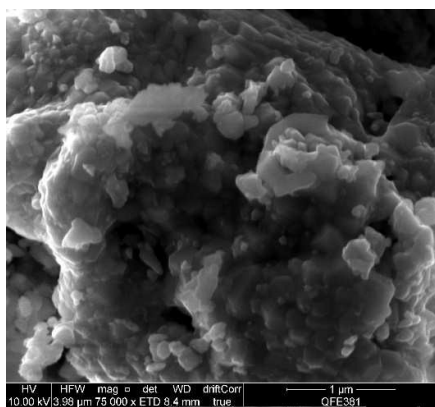
Fig. 5 – Scanning Electron Micrograph of LSMO40.
