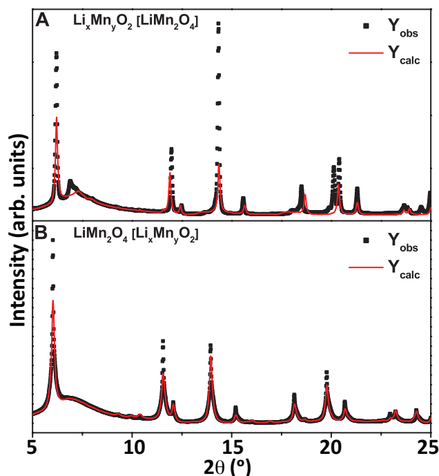
Figure 6. top) LMO-5h-15 refined with the \text{LiMn}_2\text{O}_4 model bottom) LMO-5h refined with the \text{Li}_x\text{Mn}_y\text{O}_2 model.
