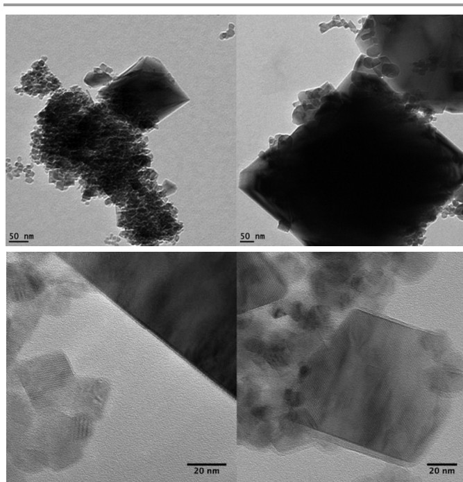
Figure 10. (Top left) LMO-4.3h, (Top Right) LMO-48h, Two bottom micrographs show HR-TEM images of the LMO-24h sample, the contrast differences at the edges may be an indication of high defect concentrations or partial reduction at the surface of the particles.
