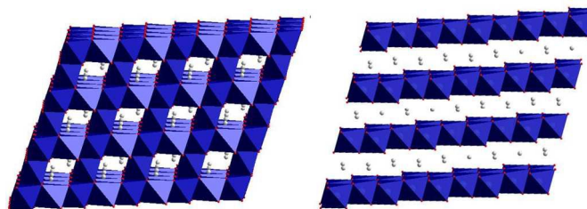
Figure 1. The crystal structures of (left) spinel LiMn 2 O 4 and (right) Li x Mn y O 2 depicted with blue [MnO 6 ]-octahedra
