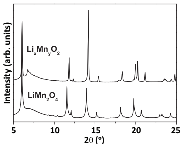
Figure 5. Synchrotron PXRD of samples (top) LMO-5h-15 and (bottom) LMO-5h. The higher LiOH content in the precursor in LMO-5h-15 results in crystallization in the layered R-3m space group instead of the spinel Fd-3m space group.
