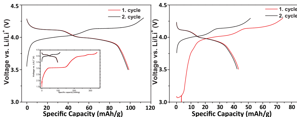
Figure 11. Voltage versus capacity curves for the first two cycles of LMO-4.3h (left) and LMO-48h (right) discharged between 3.5V and 4.3V at C/10.
