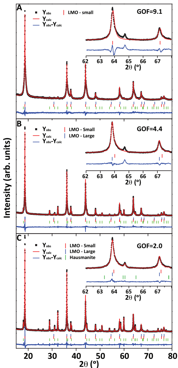
Figure 4. Rietveld Refinement of optimized in-house data on LMO-24h containing ~40% hausmannite. Fits using three different models are shown. A) single Fd-3m phase B) two Fd-3m phases with different sizes C) two Fd-3m and the hausmannite phases.
