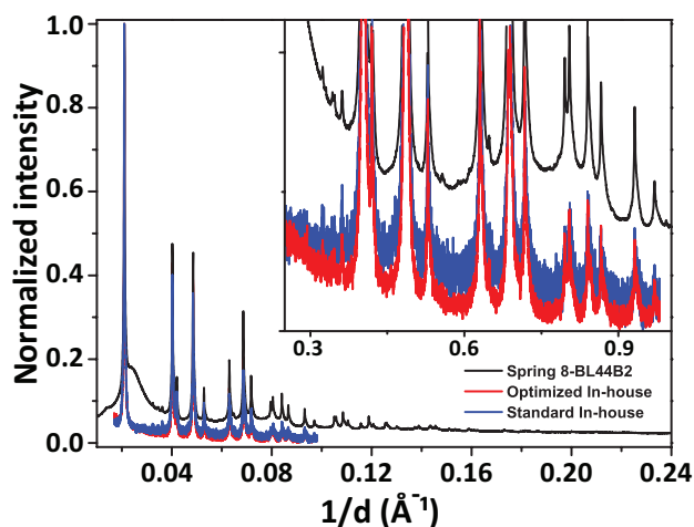
Figure 2. PXRD patterns collected with different setups, illustrating the differences in data quality achievable. The sample is in all three cases LMO-5h
