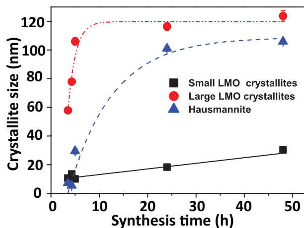
Figure 9. Crystallite size from refinement as a function of synthesis time.
