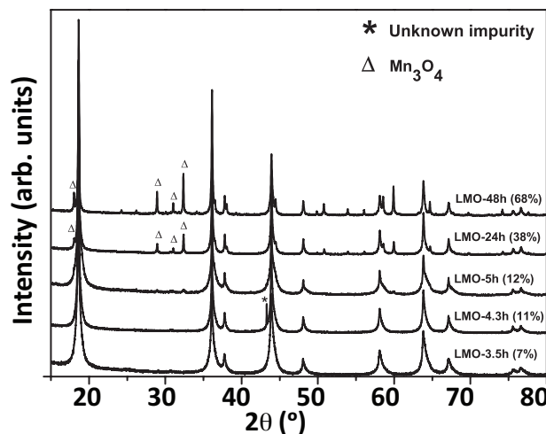
Figure 7. PXRD patterns of all samples synthesized with varying reaction time. The \text{Mn}_3\text{O}_4 content extracted via Rietveld refinement is given in parentheses. The data were collected using the optimized in-house setup.
