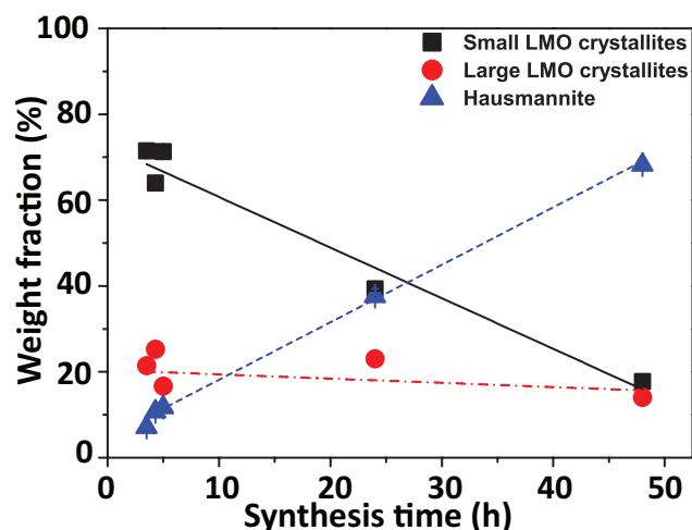
Figure 8. Weight fraction from refinements as a function of synthesis time, lines are solely ment to act as guides to the eye.
