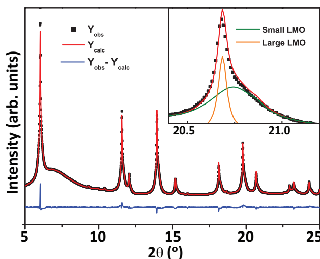
Figure 3. Rietveld refinement of the Spring8-BL44B2 data of sample LMO-5h, the insert shows the contribution of both LMO phases to the bimodal crystallite size distribution
