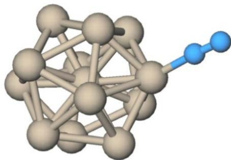
Fig. 2: Computed geometry of [\text{Co}_{13}(\text{N}_2)_1]^+ . The assumed icosahedral \text{Co}_{13}^+ core is a low lying stable geometry, and it only physisorbs \text{N}_2 in \mu_1 head-on coordination. Note, that all cobalt surface atoms are equivalent, thus giving rise to a single IR active N-N stretching vibration at about 2230 \text{cm}^{-1} (scaled by 0.95) with variations by spin multiplicity of the cobalt cluster core (likely 2S + 1 = 25, 27, 29, 31 ) (See text for discussion).
