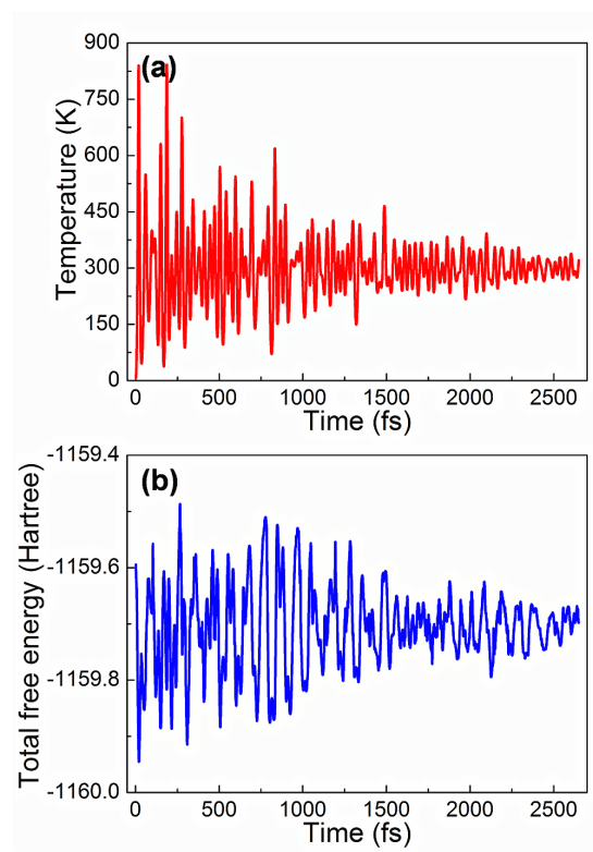
Fig. 4 (Color online) (a) kinetic temperature and (b) total free energy along the AIMD trajectory for the ACPNR ( P_{180} ). The simulation is performed for 2.5 ps at 300 K.
