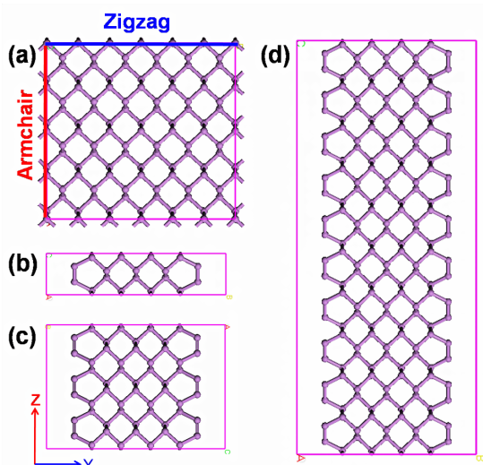
Fig. 2 (Color online) Geometric structures of (a) 2D phosphorene in the 1 \times 6 \times 4 supercell and different 1D ACPNRs with a width N = 4 in the (b) unit cell ( P_{18} ), (c) 1 \times 1 \times 3 ( P_{54} ) and (d) 1 \times 1 \times 10 ( P_{180} ) supercells. The violet balls denote phosphorus atoms. Two types of edges, armchair and zigzag, are highlighted in the insert.
