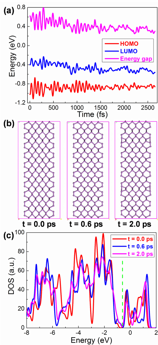
Fig. 5 (Color online) (a) HOMO, LUMO and energy gap for the ACPNR ( P_{180} ) along the AIMD trajectory. (b) Geometric structures and (c) density of states (DOS) at three snapshots of the simulation at t = 0.0 , 0.6 and 2.0 ps. The Fermi level is marked by the green dotted line.
