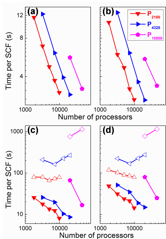
Fig. 3 (Color online) The change of wall clock time with respect to the number of processors used for the computation for three ACPNR systems of different sizes (P 2160 , P 4320 and P 10800 ). (a) Strong scaling of the generation of ALB functions step, (b) strong scaling of the DG Hamiltonian matrix construction step, (c) strong scaling of the evaluation of the approximate charge density, energy and forces from the constructed DG Hamiltonian matrix, (d) strong scaling of the overall computation. The reported wall clock time is for one SCF iteration. The timing and scaling shown in (c) and (d) depend on whether DIAG (hollow markers) or PEXSI (solid markers) is used to evaluate physical quantities such as charge density, energy and forces.
