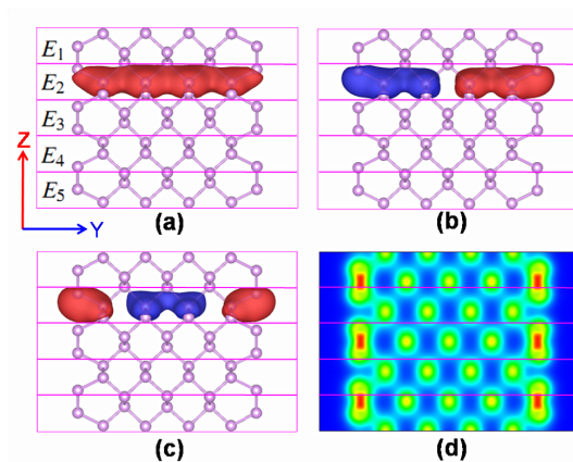
Fig. 1 (Color online) The isosurface of the first three ALB functions, (a) \phi_1 , (b) \phi_2 , (c) \phi_3 , belonging to the second element and (d) the electron density \rho across the YZ plane in the global domain in the example of P_{54} . There are 5 elements and 160 ALB functions in each element in the P_{54} system.
