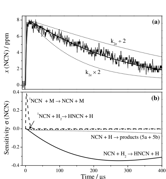
Fig. 1 (a) Typical experimental NCN concentration-time profile in comparison with numerical simulations. T = 1582 K, p = 544 mbar, \rho = 4.13 \times 10^{-6} mol/cm 3 , [\text{H}_2] = 4.0\% , [\text{NCN}_3] = 8.2 ppm, k_{2e}(\text{NCN} + \text{H}_2 \rightarrow \text{HNCN} + \text{H}) = 1.8 \times 10^{10} cm 3 mol -1 s -1 (best fit, solid curve). (b) Corresponding sensitivity analysis for NCN.
