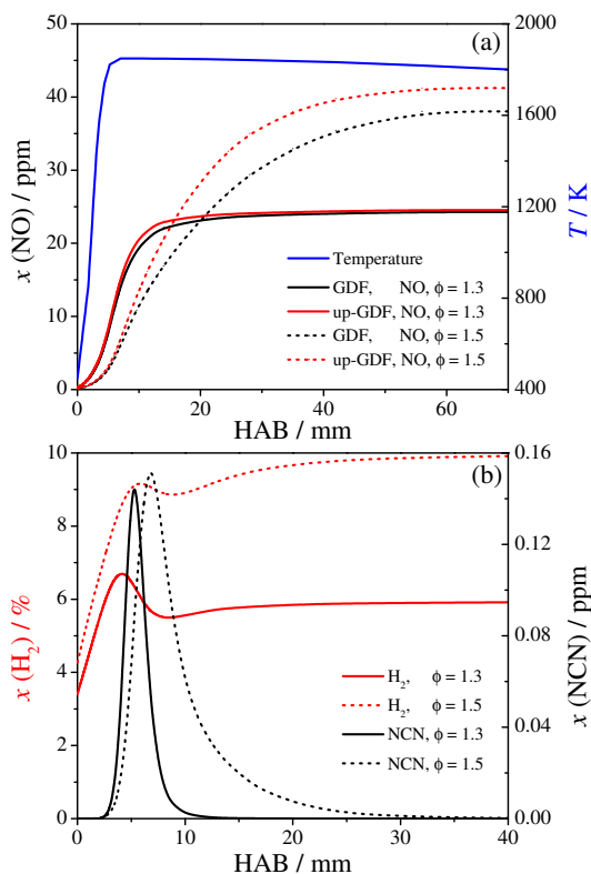
Fig. 4 a) NO profiles simulated for the low pressure flames (see text) at a richness of \phi = 1.3 and \phi = 1.5 . Results are shown for both the GDF and up-GDF mechanisms. b) Corresponding \text{H}_2 and NCN profiles simulated with the up-GDF mechanism.
