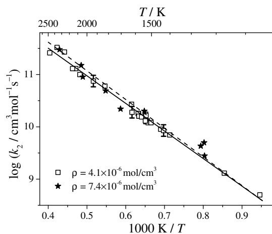
Fig. 3 Arrhenius plot of the rate constant for the reaction NCN + H 2 → products. Experimental data at two different total densities \rho \approx 4.1 \times 10^{-6} mol/cm 3 (open squares) and \rho \approx 7.4 \times 10^{-6} mol/cm 3 (star symbols) and corresponding Arrhenius fit (solid line) for an evaluation assuming radical products (channel (2c)-(g)) are shown. The dashed line depicts an Arrhenius fit obtained for an alternative data evaluation (corresponding data points are not shown) assuming stable reaction products (channels (2a) and (2b)).
