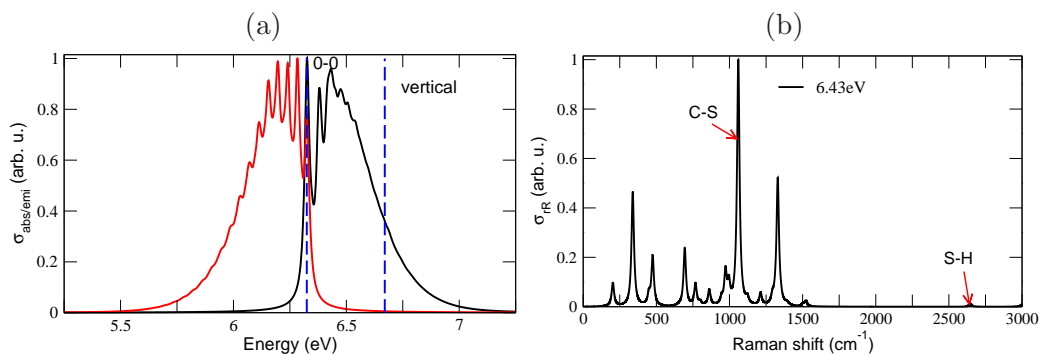
FIG. 6. (a) Absorption and emission spectra of adamantane-1-thiol, calculated using B3LYP/TZVP/IMDHOFAD and \Gamma = 100 \text{ cm}^{-1} . (b) The corresponding resonance Raman spectrum, calculated with an excitation energy of 6.43 eV. Broadening factor \tilde{\Gamma} = 100 \text{ cm}^{-1} , and resulting stick spectra were broadened by Lorentzians of FWHM 10 \text{ cm}^{-1} . Two relevant peaks are indicated by arrows (see text).
