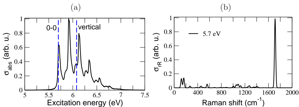
FIG. 4. (a) Absorption spectrum of Ada=Dia=Ada, calculated using B3LYP/6-31G*/IMDHO (STA) and \Gamma = 100 \text{ cm}^{-1} . (b) The corresponding resonance Raman spectrum, calculated with an excitation energy of 5.7 eV. Broadening factor \tilde{\Gamma} = 100 \text{ cm}^{-1} , and resulting stick spectra were broadened by Lorentzians of FWHM 10 \text{ cm}^{-1} .
