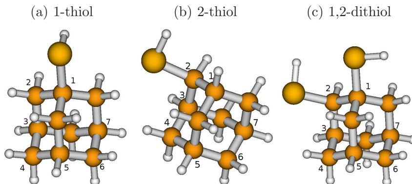
FIG. 5. The geometries of the optimized S_0 states of three isomers of adamantane-1-thiol (a) and adamantane-2-thiol (b), both C_{10}H_{15}SH , as well as adamantane-1,2-dithiol (c), C_{10}H_{14}(SH)_2 , obtained at the B3LYP/TZVP level of theory. The large yellow balls represent the S atoms, while the smaller brown balls and the white balls represent the C and H atoms respectively.
