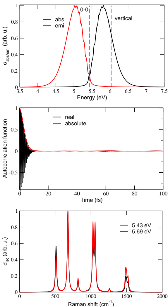
FIG. 10. The vibrationally resolved absorption and emission spectra (upper panel) for urotropine. Vertical dashed lines stand for 0-0 and vertical (for absorption) transitions, respectively. The middle panel shows the corresponding autocorrelation function for absorption. For both upper panels damping factors \Gamma = 200 \text{ cm}^{-1} have been used. Resonance Raman spectra at selected excitation energies \omega_L are shown in the lower panel. In this case, a broadening factor \tilde{\Gamma} = 200 \text{ cm}^{-1} has been used and the resulting stick spectrum was broadened by normalized Lorentzians of FWHM of 10 \text{ cm}^{-1} . All calculations were at the (TD-)B3LYP/TZVP/IMDHOFAD level of theory.
