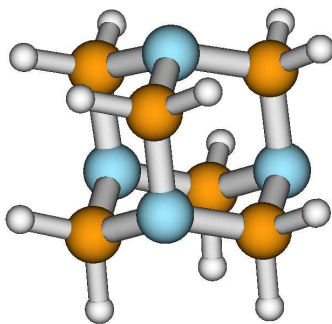
FIG. 9. The B3LYP/TZVP optimized ground state geometry of urotropine. The blue balls represent the N atoms, the brown balls the C atoms and the white balls represent the H atoms. The C-N and C-H bond lengths are 1.47 Å and 1.09 Å. The C-N-C and H-C-H bond angles are around 108°, while the N-C-N bond angles are 112.4°. Bond lengths and angles involving similar atoms are equal.
