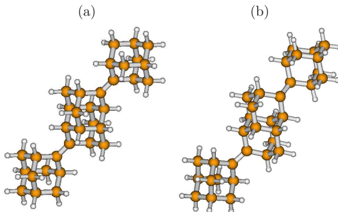
FIG. 3. The minimum geometries of the (a) S_0 and (b) S_1 electronic states of Ada=Dia=Ada, calculated at the B3LYP/6-31G* level of theory. In the S_1 state, the adamantane unit in the extreme right undergoes a rotation about the C=C bond joining it to the adjacent diamantane unit.
