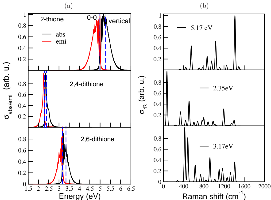
FIG. 8. (a) The vibronic absorption and emission spectra of the diamondoid thiones studied here, calculated at the B3LYP/TZVP level of theory, using the IMDHO (STA) model. From top to bottom the spectra are in the order: adamantane-2-thione, adamantane-2,4-dithione and adamantane-2,6-dithione. The dashed blue lines represent the 0-0 and vertical transition energies for all three plots. (b) The corresponding rR spectra, using the same model. The excitation energies \omega_L are also indicated and correspond to \Delta E_{\text{vibro}} of each molecule. Broadening parameter of \Gamma and \tilde{\Gamma} = 100 \text{ cm}^{-1} were used. For rR, resulting stick spectra were broadened by Lorentzians with FWHM of 10 \text{ cm}^{-1} .
