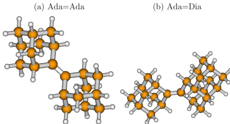
FIG. 1. The optimized geometries at the ground electronic states ( S_0 , g) of Ada=Ada (a) and Ada=Dia (b), at the B3LYP/TZVP level of theory. Brown balls represent the C atoms and the white balls H atoms. The central bond joining the two diamondoid units is a C=C double bond, with a bond length of 1.34 Å for either. Other C-C bonds are single, with bond lengths typically of 1.54 Å. The C=C bond-length compares well with recently available experimental (1.34 Å for Ada=Ada and 1.33 Å for Ada=Dia) and theoretical (DFT and MP2) data [36]. The calculated C-H bond lengths (1.09 Å) also show good agreement with the corresponding experimental data.
