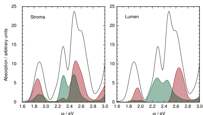
Fig. 6 LHC-II monomer TDDFT spectrum. Contribution from Chl at stromal side (left) and luminal side (right) of the membrane. Chl a are in red and Chl b in green, the gray line shows the calculated spectrum for the full monomer chlorophyll network. Individual Chl contributions are summed to give the curves shown here.
