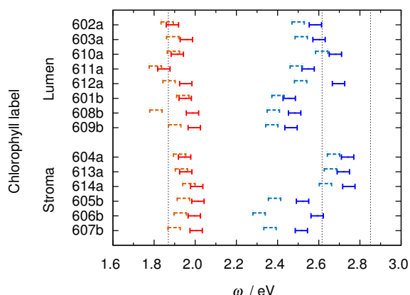
Fig. 2 Distribution of peak energies in Chl TDDFT spectra. Q-band excitations occur between 1.9–2.0 eV and those of the Soret-band between 2.5–2.9 eV. Chl numbering taken from PDB file 1RWT. Solid lines correspond to isolated Chl spectra and dashed lines to spectra of the individual Chl within the LHC-II monomer Chl network, calculated using our local-dipole method. Vertical lines indicate the position of the maxima of the Q- (1.86 eV) and Soret-band (2.62 and 2.85 eV) found experimentally. 43
