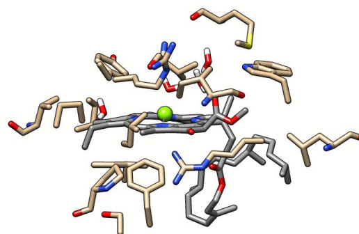
Fig. 3 Model system used in evaluation of effect of protein environment on chlorophyll absorption spectrum. Chlorophyll 608b carbons shown in grey, amino acid side chain carbons in brown. Except for water molecules, all hydrogen atoms are omitted to aid visualisation. This Chl was selected because of its more complete protein surroundings as compared with other Chl which overlapped significantly with neighboring chromophores (Figure S9).
