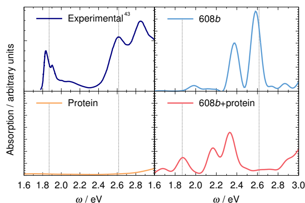
Fig. 4 Effect of inclusion of surrounding amino acid residues on the spectrum of Chl 608b. Vertical lines indicate the experimental position of the Q-band (1.86 eV) and Chl b component of the Soret-band (2.62 eV). 43
