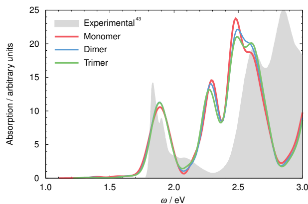
Fig. 5 LHC-II monomer (red), dimer (blue) and trimer (green) TDDFT spectrum. The absorption intensities of the dimer has been scaled by half and the trimer by one third to aid in comparison of the spectra. The filled gray curve is the experimental absorption spectrum of LHC-II. 43 Here the lower absolute accuracy of TDDFT for the predominantly multi-electron Soret-band excitation energies (discussed above) can be seen.
