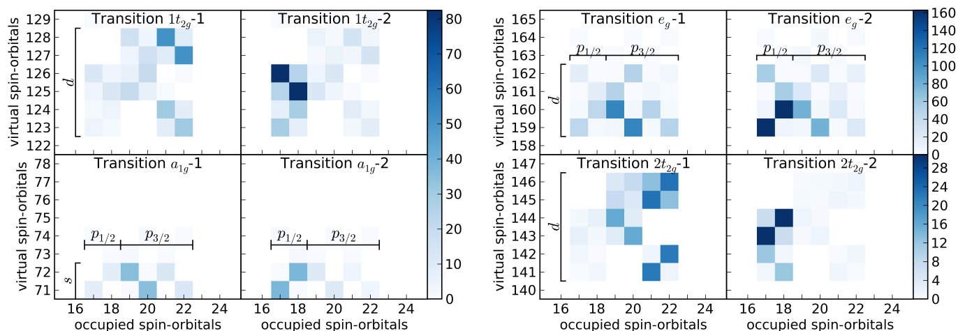
Fig. 2 The DWTA analysis of the first eight dominant transitions in the XANES spectrum of \text{SF}_6 — a_{1g} (bottom left), 1t_{2g} (top left), 2t_{2g} (bottom right) and e_g (top right). The intensity of the blue color corresponds to the intensity of the particular excitation; the units in the colorbars on the right are arbitrary — only relative intensities are meaningful. The excitations are always Kramers-paired and form 2 \times 2 sub-matrices. Due to an ambiguity in the phase of these spin-orbitals the internal structure of the 2 \times 2 sub-matrices does not have a physical interpretation.
