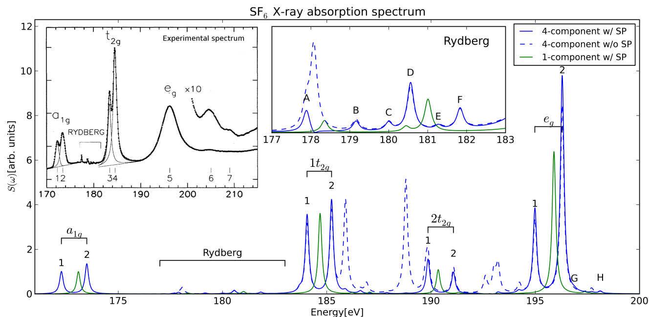
Fig. 1 The photoabsorption spectrum of \text{SF}_6 near the sulfur L_{2,3} -edges. Fourier-transformed data was fitted using Lorentzian functions to obtain the spectrum; the normalization is the same as in experiment. Continuous lines: results of the calculations with the selective perturbation (SP) restricted only to core sulfur 2p_{1/2} and 2p_{3/2} spin-orbitals. Dashed line: results of the calculation with the full perturbation. Peaks without a label represent excitations from non-core occupied orbitals to high-lying virtual spin-orbitals.
