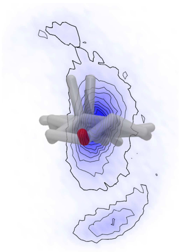
Figure 7. Distribution of the C25 position when looking at cholesterol from the top (looking at the OH group (red) towards the aliphatic side chain along the main rotational axis of cholesterol). Hydrogens were omitted from the cholesterol structure for clarity and the two \text{CH}_3 groups that stick out of the plane of the cholesterol rings can be seen pointing upwards. The probability distribution of the C25 position is indicated by blue color, where more intense color corresponds to higher probability.
