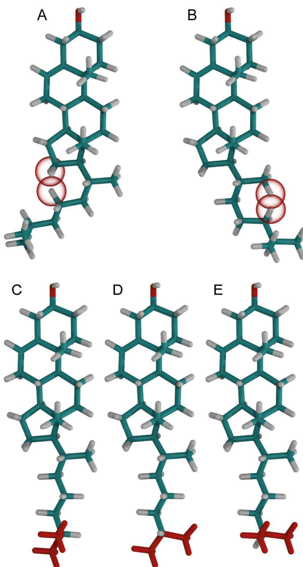
Figure 4. Cholesterol structures with various dihedral angles, where hydrogens that have the closest steric contact are highlighted by a red sphere with the van der Waals radius of hydrogen. All dihedral angles were in their most likely conformation with the exception of (A) C17-C20-C22-C23 at -60^\circ , (B) C20-C22-C23-C24 at -60^\circ , (C) C23-C24-C25-C26 at +60^\circ , (D) C23-C24-C25-C26 at 180^\circ , and (E) C23-C24-C25-C26 at -60^\circ respectively. In panels (C), (D), and (E) the two terminal \text{CH}_3 groups were colored red for better visibility.
