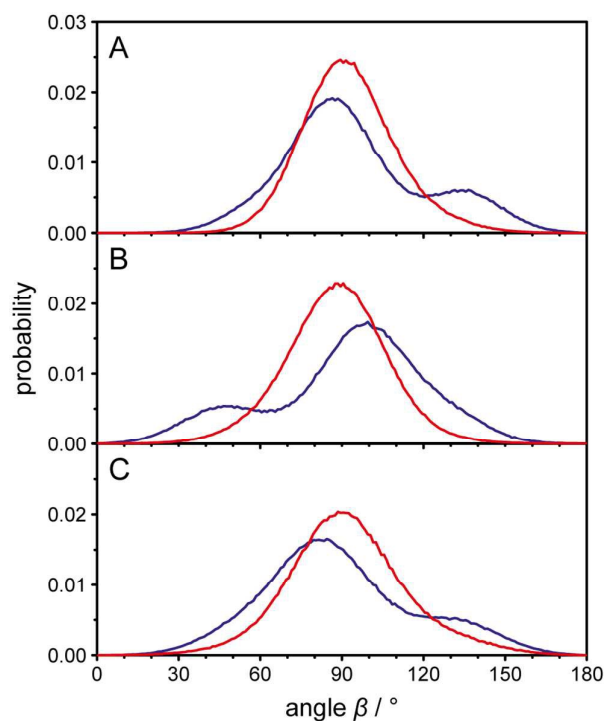
Figure 2. (A) Histograms of the angle \beta between the two carbon hydrogen bonds attached to C22 and the membrane normal as obtained from the MD simulation of POPC/cholesterol (3:1 mol/mol) at 37°C. Panels (B) and (C) show the same histograms for C23 and C24, respectively. The data for hydrogen A is shown in blue and for hydrogen B in red.
