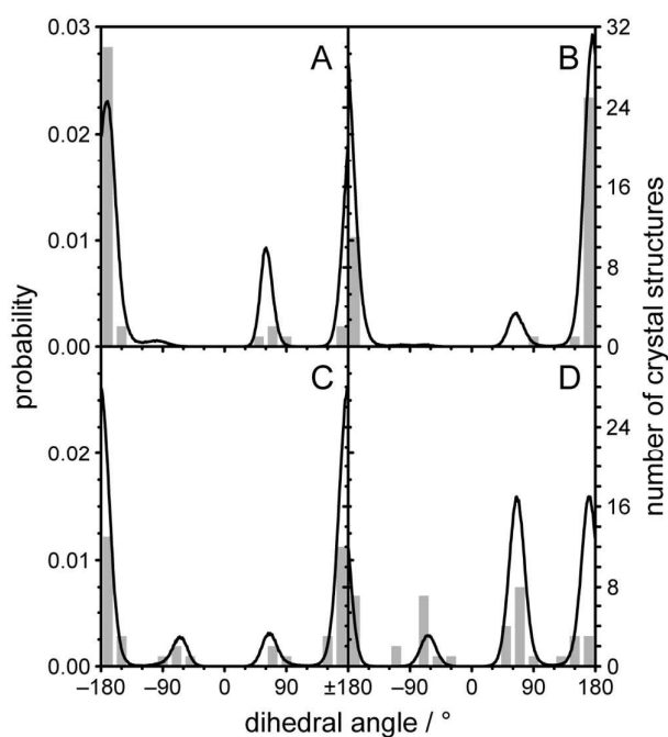
Figure 3. Histograms of dihedral angles in the aliphatic chain of cholesterol as obtained from the MD simulation of POPC/cholesterol (3:1 mol/mol) at 37°C and from 38 crystal structures found in the literature 46-49 for (A) C17-C20-C22-C23, (B) C20-C22-C23-C24, (C) C22-C23-C24-C25, and (D) C23-C24-C25-C26. Data from the MD simulation is shown as black lines while data from the crystal structures is shown as grey bars.
