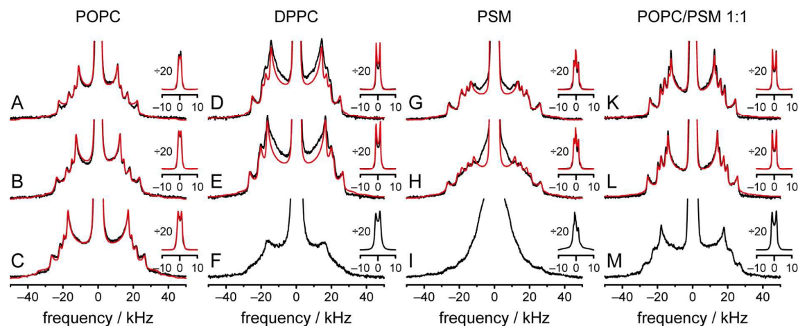
Figure 6. ^2\text{H} NMR spectra of cholesterol- d_{11} (25 mol% relative to all other lipids) in various environments at 50°C (A, D, G, K), 37°C (B, E, H, L), and 5°C (C, F, I, M). NMR spectra were measured in POPC (A, B, C), DPPC (D, E, F), PSM (G, H, I) and POPC/PSM (1:1 mol/mol) (K, L, M). The inset shows the same spectra vertically divided by a factor of 20 to show the intense Pake doublets from the two terminal \text{CH}_3 groups. Measured spectra are shown in black, while numerical fits are red.
