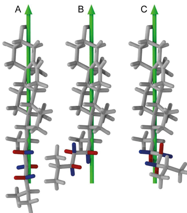
Figure 5. Cholesterol structures with the dihedral angle C17-C20-C22-C23 in (A) 180^\circ , (B) +60^\circ , and the prohibited (C) -60^\circ orientation respectively. The green arrow indicates the main rotational axis of cholesterol while A hydrogens at C22, C23, and C24 are colored blue and B hydrogens are colored red.
