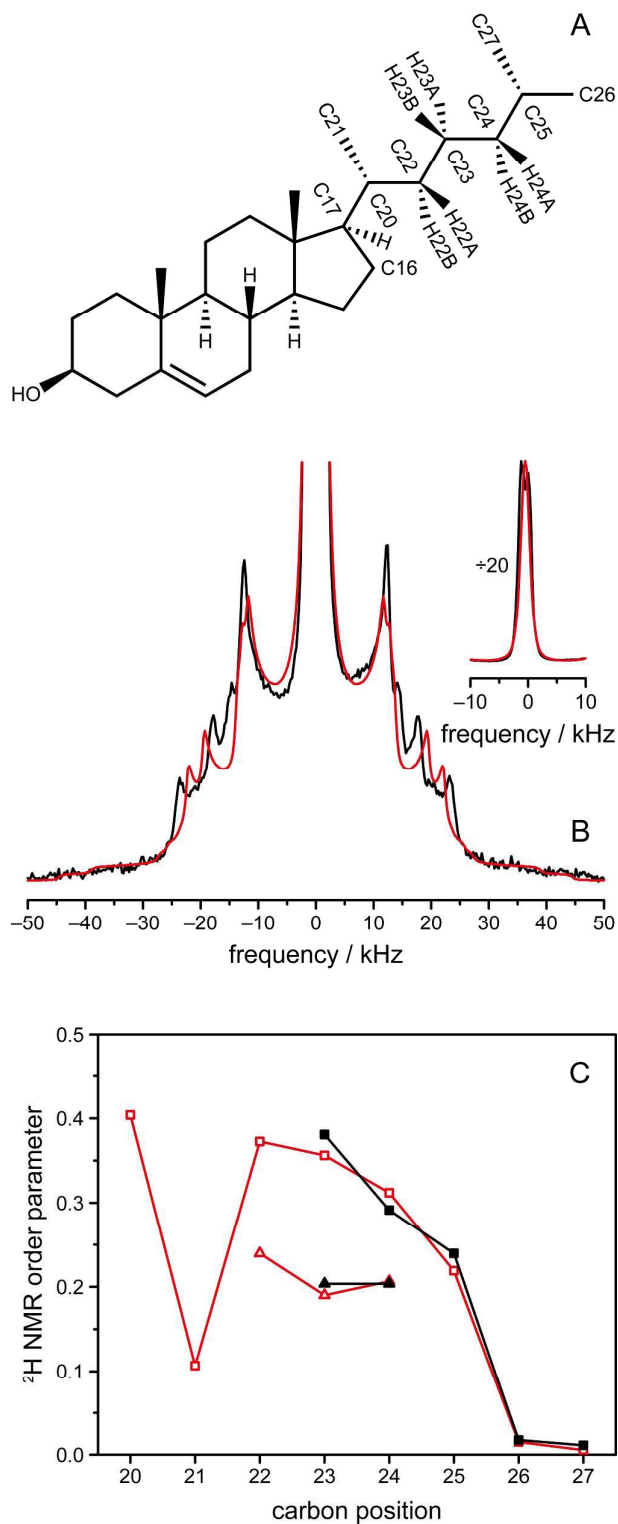
Figure 1. (A) Chemical structure of cholesterol including the relevant nomenclature. In cholesterol- d_{11} , hydrogens were replaced by deuterium at positions C23, C24, C25, C26, and C27. (B) ^2\text{H} NMR spectra of POPC/cholesterol- d_{11} (3:1 mol/mol) at 37°C. The experimentally obtained ^2\text{H} NMR spectrum is shown in black, while the spectrum calculated
