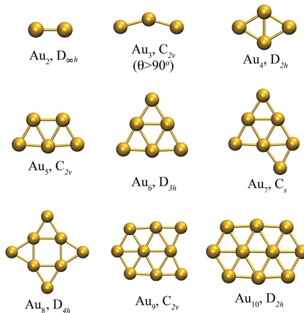
Figure 1: Global minimum energy structures studied for Au 2 -Au 10 clusters, showing the point group symmetries, as computed using PBE/VDB.
