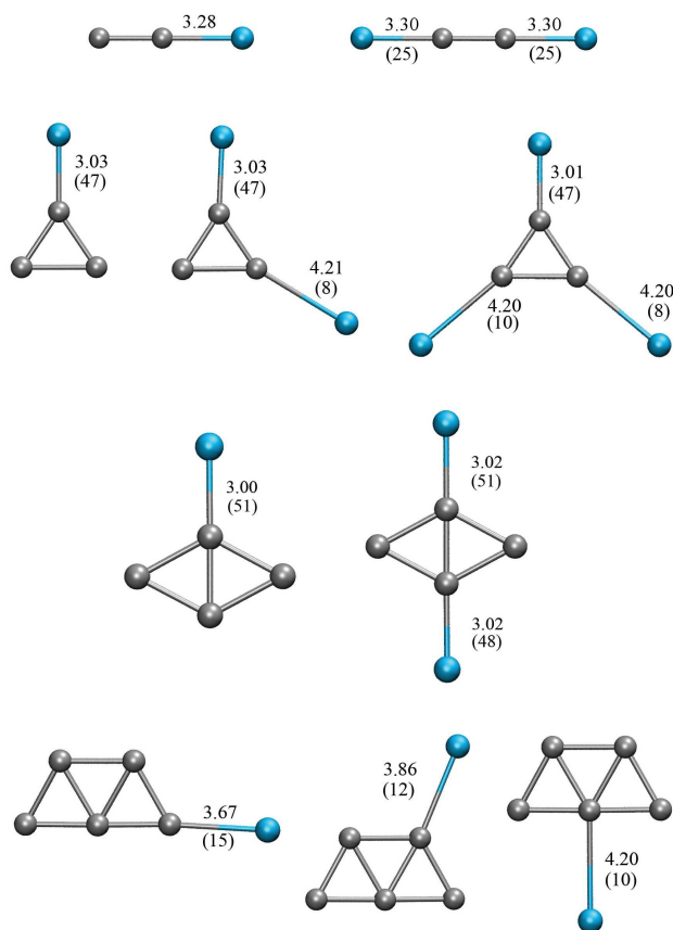
Figure 5: Various possible configurations of \text{Ag}_2\text{Ar-Ag}_5\text{Ar} complexes indicating the Ag–Ar distance and the Ar binding energy (in parenthesis) in Å and meV/atom, respectively. Results obtained using PBE/GTH.
