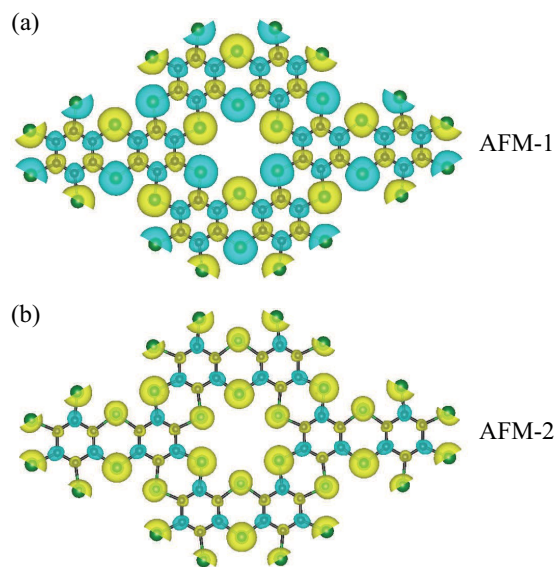
Fig. 3 (Color online) Charge density difference, \rho_{up}-\rho_{down} , of C_2As monolayer structure for (a) fully anti-ferromagnetic (AFM-1) order and (b) anti-ferromagnetic order in the benzene ring (AFM-2) where green/yellow color is for minority/majority spin states. The plotted isosurface values are 10^{-3} e/\text{\AA}^3 and 10^{-5} e/\text{\AA}^3 for (a) and (b) respectively.
