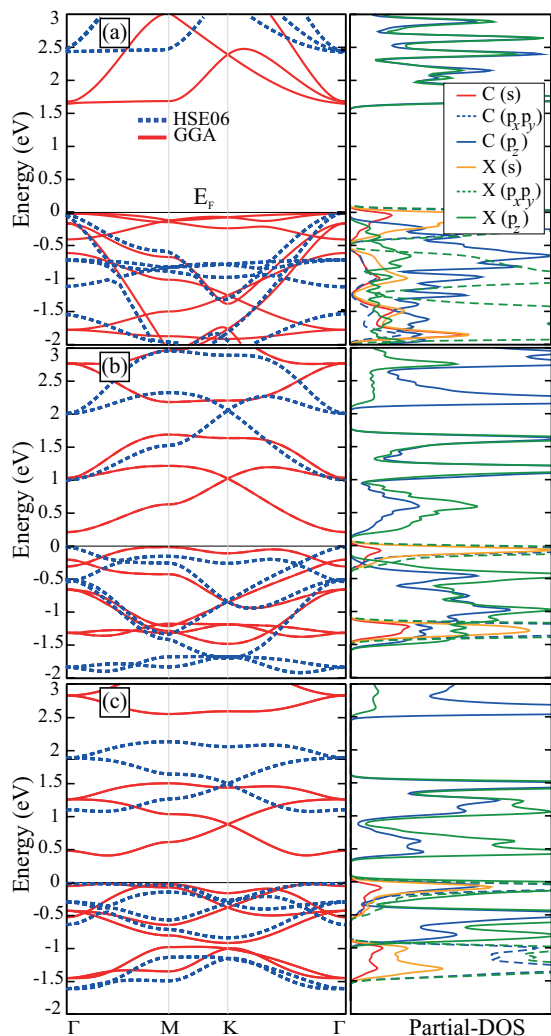
Fig. 2 Band-structures (left-panel) and corresponding partial density of states (right-panel) of (a) C_2N (b) C_2P , and (c) C_2As where red curves are for bands calculated within GGA approximation while dashed blue curves are for bands calculated within HSE06 on top of GGA. The Fermi energy ( E_F ) level is set to the valence band maximum.
