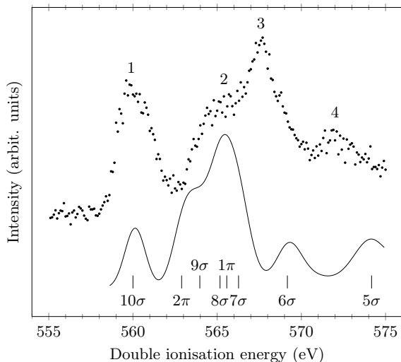
FIG. 4. Experimental core-valence double photoionisation spectrum of acetaldehyde reflecting the formation of O1s^{-1}v^{-1} states recorded at the photon energy of 600 eV, shown as dots. The single valence photoelectron spectrum measured by Keane et al. 20 , convoluted with a Gaussian function of 1.4 eV width (FWHM) and shifted by 549.77 eV is included for direct comparison. The bin size is 100 meV
