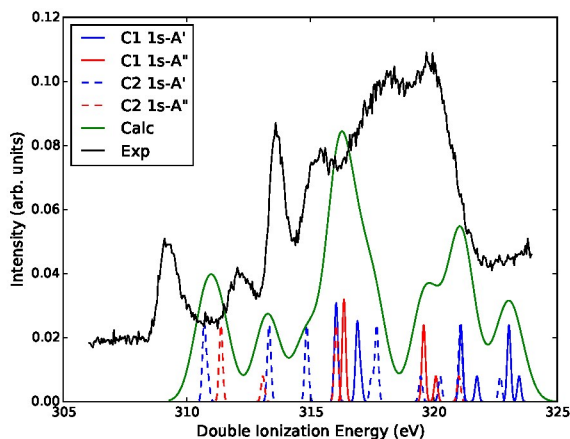
FIG. 5. Results of the Z+1 approximation for C1s^{-1}v^1 .
