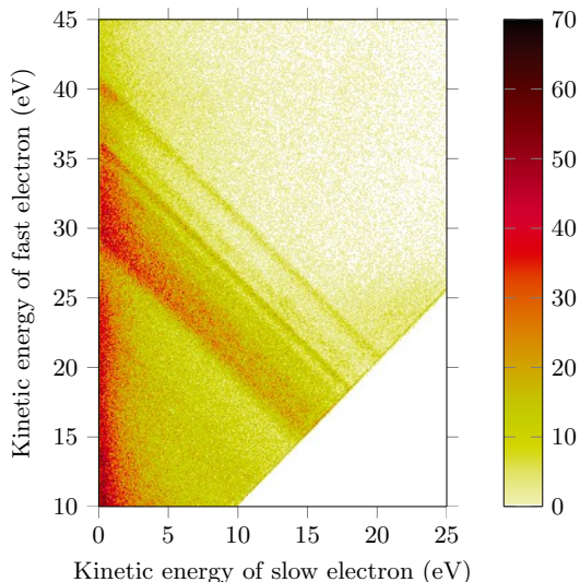
FIG. 1. Coincidence map of acetaldehyde formed by electron pairs detected in coincidence with thirdly emitted carbon Auger electrons. The data were obtained at the photon energy of 350 eV. The straight diagonal lines reflect the formation of C1s^{-1}v^{-1} states. The bin size is 100 meV.
