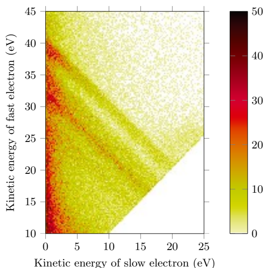
FIG. 2. Coincidence map of acetaldehyde formed by electron pairs detected in coincidence with thirdly emitted oxygen Auger electrons. The data were obtained at the photon energy of 600 eV. The straight diagonal lines reflect the formation of O1s^{-1}v^{-1} states. The bin size is 200 meV.
