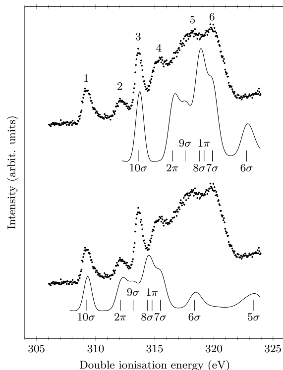
FIG. 3. Experimental core-valence double ionisation spectrum of acetaldehyde reflecting the formation of C1s^{-1}v^{-1} states recorded at the photon energy of 350 eV, shown as dots. The single valence photoelectron spectrum measured by Keane et al. 20 , convoluted with a Gaussian function of 0.7 eV width (FWHM) and shifted by 298.97 eV (lower panel) and 303.37 eV (upper panel), respectively, is included for direct comparison. The bin size is 50 meV
