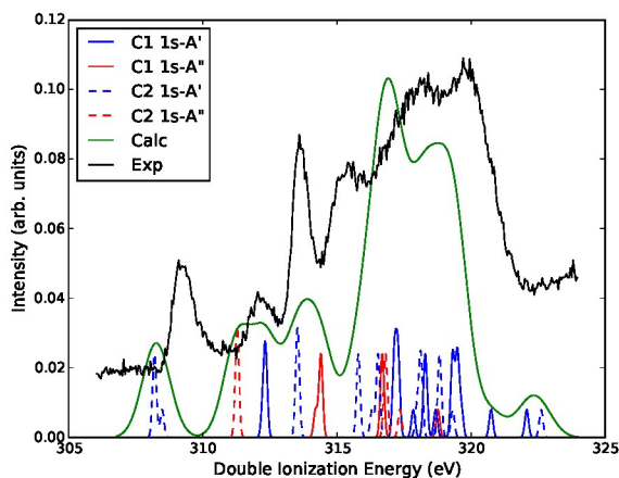
FIG. 7. MCSCF results of C1s^{-1}v^1 .
