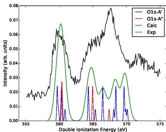
FIG. 13. SDCI results of O1s^{-1}v^1 .
