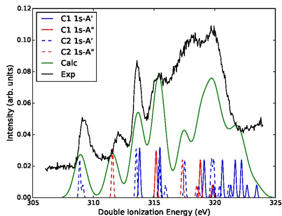
FIG. 8. SDCI results of C1s^{-1}v^1 .
