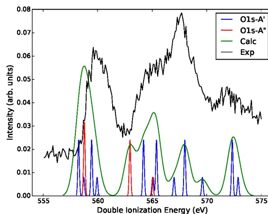
FIG. 11. Hartree-Fock results of O1s^{-1}v^1 .
