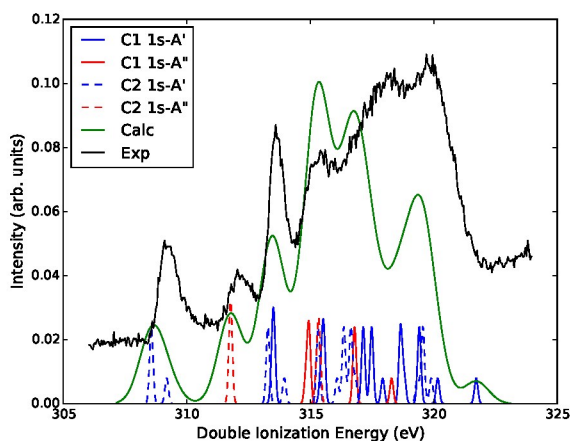
FIG. 9. CASPT2 results of C1s^{-1}v^1 .
