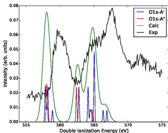
FIG. 14. CASPT2 results of O1s^{-1}v^1 .
