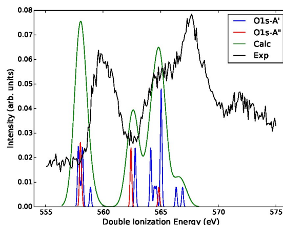
FIG. 12. MCSCF results of O1s^{-1}v^1 .
