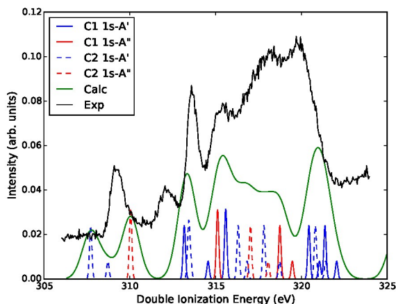
FIG. 6. Hartree-Fock results of C1s^{-1}v^1 .
