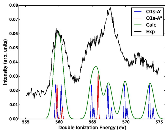
FIG. 10. Results of the Z+1 approximation for O1s^{-1}v^1 .
