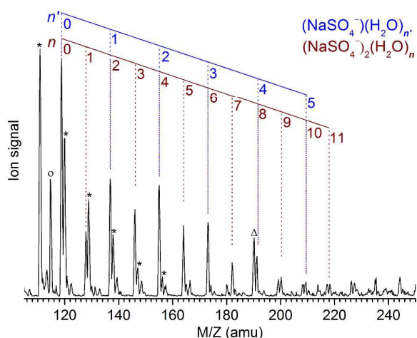
Fig. 1 Mass spectrum of a 10 mM solution of \text{Na}_2\text{SO}_4 in a 1:1 water/acetonitrile solvent revealing the (\text{NaSO}_4^-)_2(\text{H}_2\text{O})_{n=0-11} and \text{NaSO}_4^-(\text{H}_2\text{O})_{k=0-5} progressions. Further contributions correspond to hydrated sulfate clusters \text{SO}_4^{2-}(\text{H}_2\text{O})_{n=7-12} (denoted with an asterisk) and \text{HSO}_4^-\text{H}_2\text{O} (circle). The mass peak at 190 amu labeled with “ \Delta ” is an unidentified impurity.
