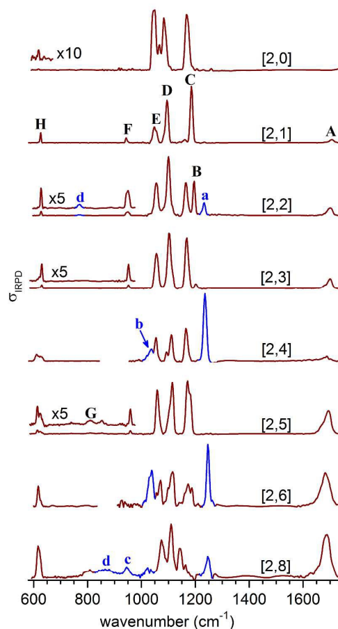
Fig. 3 IRMPD spectra of (\text{NaSO}_4^-)_2(\text{H}_2\text{O})_n complexes (red trace), denoted as [2, n ]. The photodissociation cross section \sigma_{\text{IRPD}} is plotted as a function of the wavenumber. For even n the IRMPD spectra contain spectroscopic features (blue trace and labeled with small letters) which are unambiguously attributed to the monomeric counterparts [1, k ] with k = n/2 .
