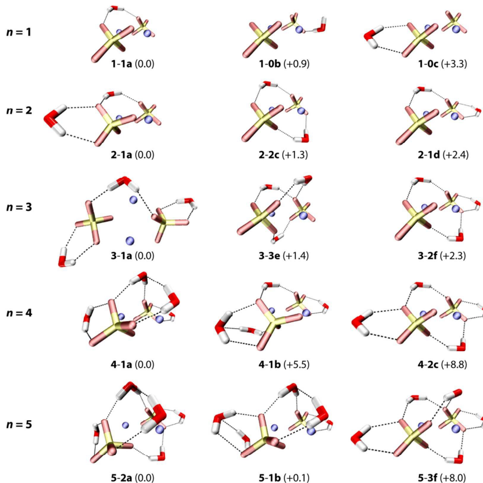
Fig. 5 B3LYP/def2-TZVP minimum-energy structures of the (NaSO_4)_2(H_2O)_n complexes with n = 1-5 . Relative energies (with ZPE correction) are given in kJ/mol.
