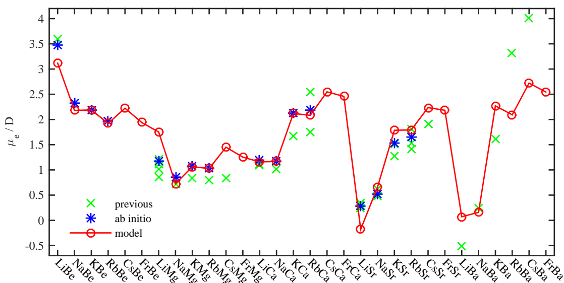
Fig. 8 Dipole moment predictions as described in the text ( \circ ). The three parameters of the model were determined by fitting to the ab initio results of this work ( * ). The resulting model shows good agreement with results from previous theoretical treatments ( x ) listed in Table 2. Additional values have been added for the CsMg (Ref. 61), CsSr (Ref. 63) and AK-Ba molecules (Ref. 64).
