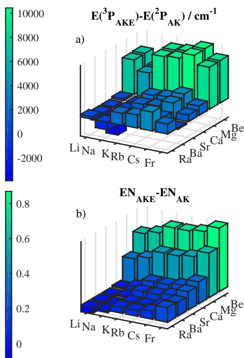
Fig. 2 Differences between AK and AKE atoms for two atomic properties are shown in the figure, in the upper plot energy differences of the first P-excitations 92 and in the lower plot the differences in the electronegativities according to Pauling's scale. 96
