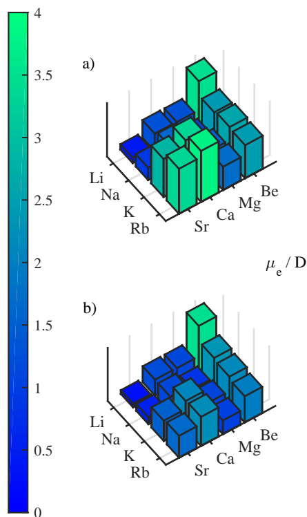
Fig. 1 The permanent electric dipole moment of the doublet ground state at its equilibrium distance, obtained at the MCSCF+MRCI level of theory, without (a) and with (b) the inclusion of core polarization potentials.
