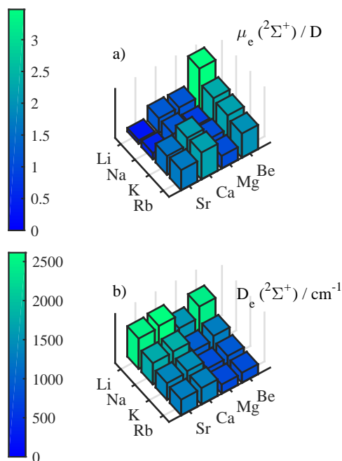
Fig. 3 The permanent electric dipole moment (a) and the potential depth (b) for several AK-AKE molecules in their ground state ( ^2\Sigma^+ ) are shown.
