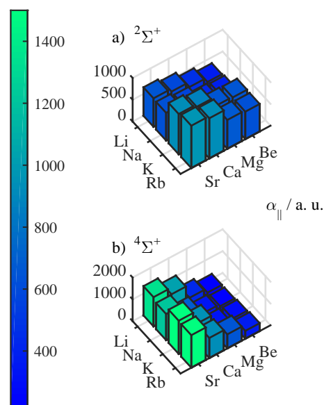
Fig. 5 Finite-field polarizabilities in the doublet ground state (upper graphics) and the lowest quartet state (lower graphics), calculated at the corresponding equilibrium geometry.
