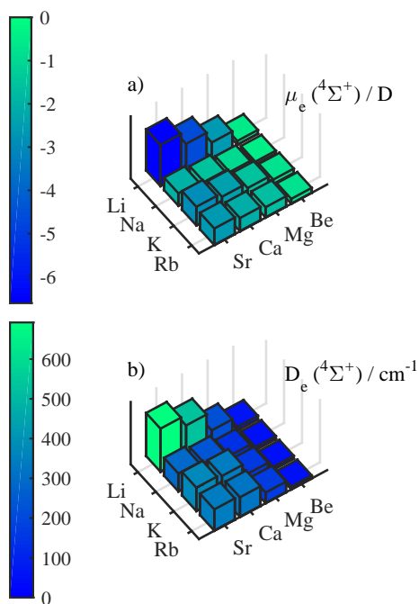
Fig. 4 The upper plot shows the PEDMs for several AK-AKE molecules in the lowest quartet state. Note that the axis is reversed so that the highest bar corresponds to the most negative value. The graphics below shows the corresponding dissociation energy for a direct comparison.
