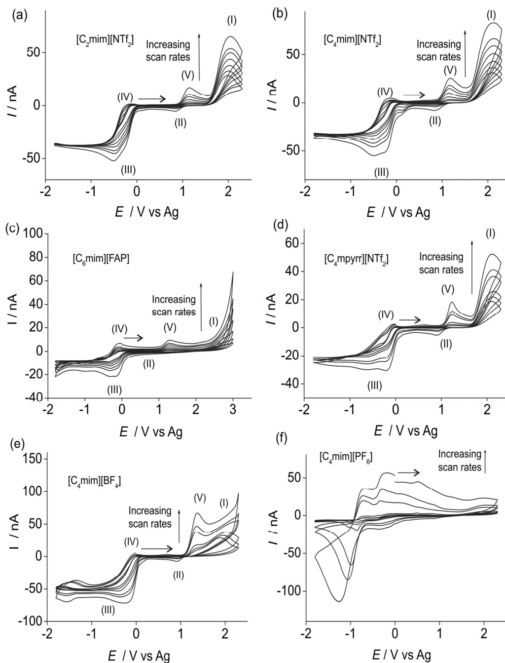
Figure 3: CVs for the oxidation (second scan) of 2.56 % hydrogen chloride gas on a 8.3 \mu m radius Pt electrode in a) [C_2mim][NTf_2] , b) [C_4mim][NTf_2] , c) [C_6mim][FAP] , d) [C_4mpyrr][NTf_2] , e) [C_4mim][BF_4] , f) [C_4mim][PF_6] at various scan rates between 0.05 and 2 V/s. The labels for peaks (I) to (V) are not included for [C_4mim][PF_6] (f) due to different reactions occurring in this RTIL.
