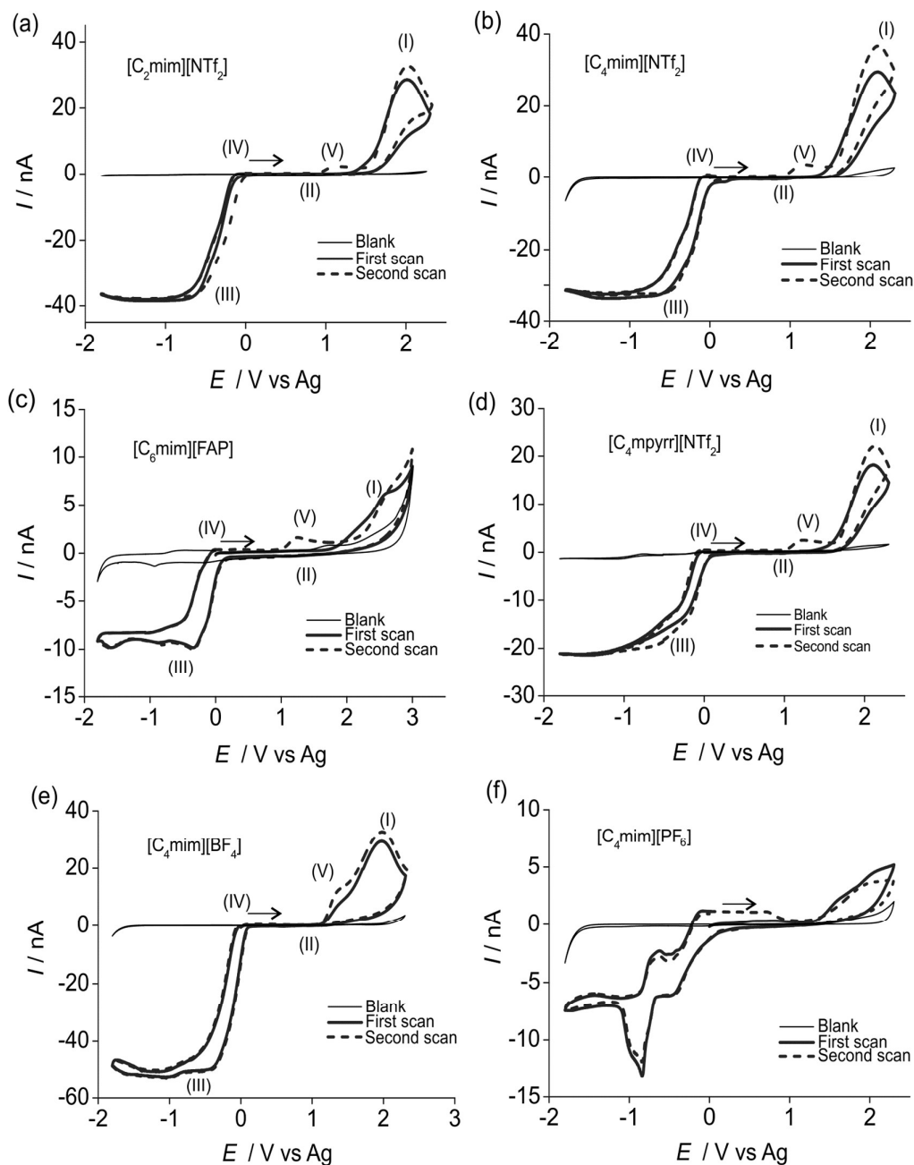
Figure 1: CVs for the oxidation of 2.56 % hydrogen chloride gas (nitrogen fill) on a 8.3 \mu\text{m} radius Pt electrode in a) [\text{C}_2\text{mim}][\text{NTf}_2] , b) [\text{C}_4\text{mim}][\text{NTf}_2] , c) [\text{C}_6\text{mim}][\text{FAP}] , d) [\text{C}_4\text{mpyr}][\text{NTf}_2] , e) [\text{C}_4\text{mim}][\text{BF}_4] and f) [\text{C}_4\text{mim}][\text{PF}_6] at a scan rate 0.1 V/s. The thick solid line is the first scan, the thick dashed line is the second scan and the thin solid line is the blank (response in the absence of hydrogen chloride gas before experiments). The labels for peaks (I) to (V) are not included for [\text{C}_4\text{mim}][\text{PF}_6] (f) due to different reactions occurring in this RTIL (see discussion).
