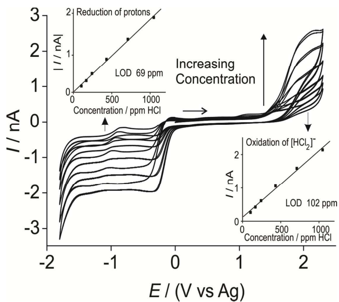
Figure 4: CVs (first and second scan) for the oxidation of different concentrations (104, 168, 242, 431, 710 and 1048 ppm) of HCl gas on a 8.3 \mu\text{m} radius Pt electrode in [C 2 mim][NTf 2 ] at a scan rate 0.1 V/s. Insets are calibration graphs of current for peak I (first scan) and peak III (first scan) vs. gas phase concentration.
