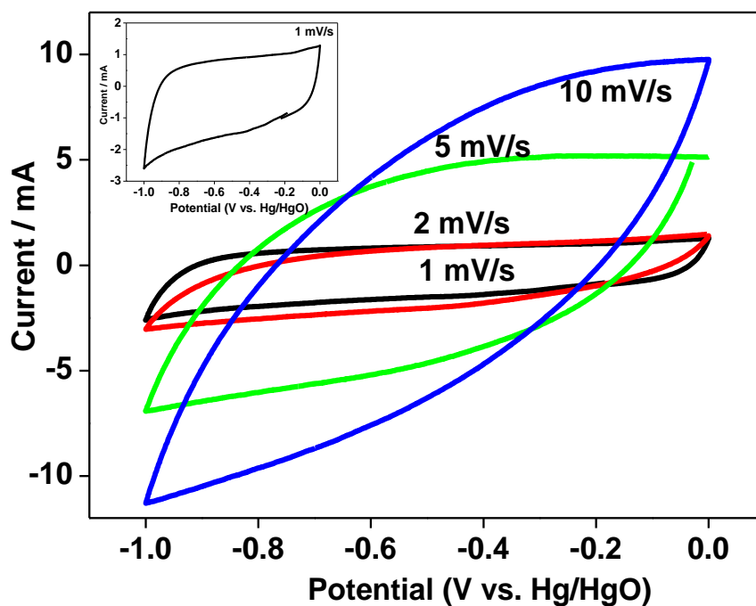
Figure 7 Cyclic voltammogram (CV) measurements of activated carbon at different scan rates. Inset is the typical electrochemical double layer capacitor (EDLC) behaviour at a low scan rate of 1 mV/s. Experiments were performed in a three-electrode system in 2M NaOH electrolyte.
