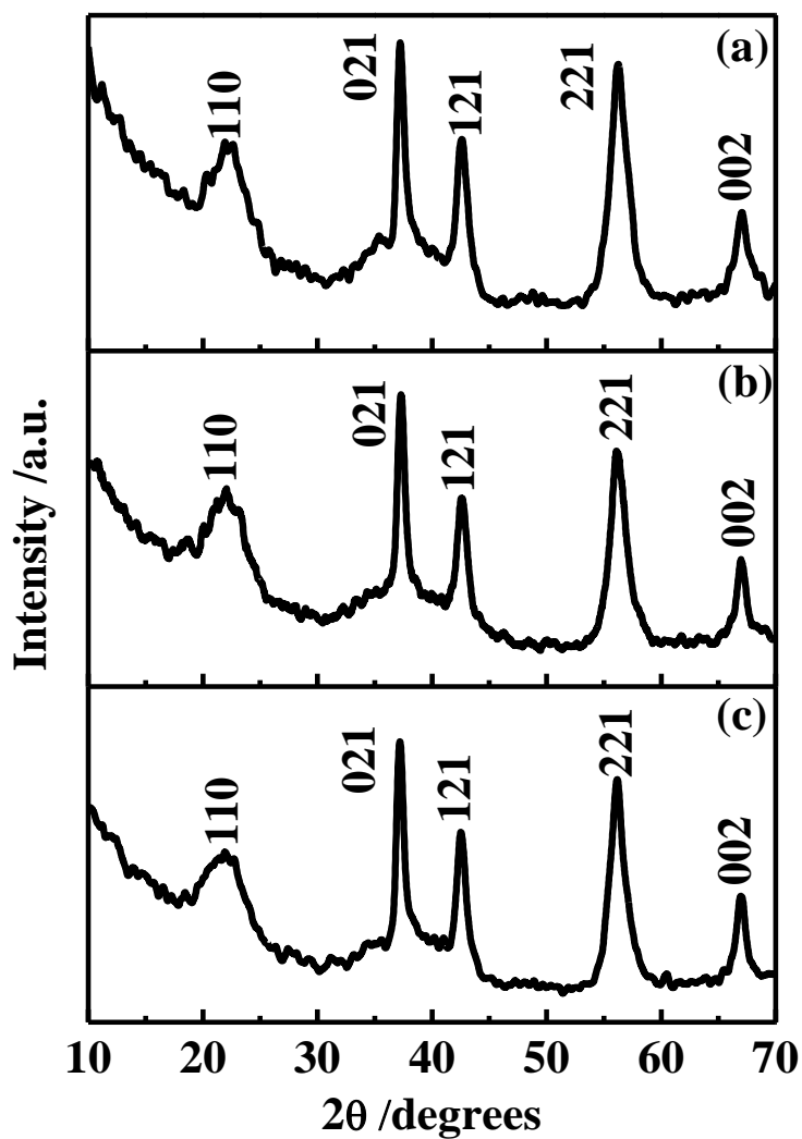
Figure 1 X-ray diffraction (XRD) patterns of the EMD materials derived from precursors (a) low-grade residue, (b) manganese cake and (c) synthetic solution.
