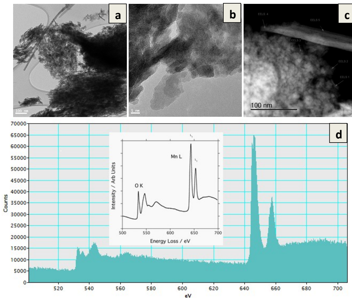
Figure 3 (a) Low magnification bright-field TEM image, (b) high resolution TEM (HRTEM), (c) high angle-annular dark field (HAADF) TEM image of fibrous structure and (d) corresponding electron energy loss spectroscopy (EELS) for EMD ( \gamma -MnO 2 ) samples derived from low-grade residue. Inset is the typical EELS spectrum for EMD.
