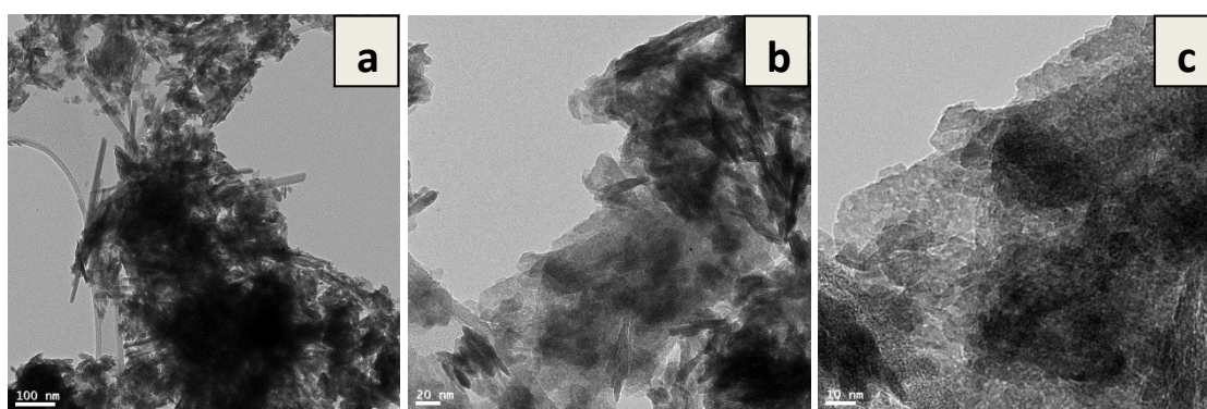
Figure 4 (a-b) Low magnification bright-field TEM, (b) detailed image of the individual particle showing rice grain shape, and (c) high resolution TEM (HRTEM) for EMD ( \gamma -MnO 2 ) samples derived from manganese cake.
