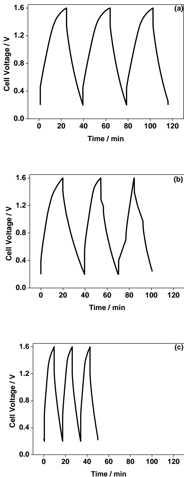
Figure 9 Charge-discharge voltage profile of the activated carbon vs. EMD asymmetric capacitor. EMD derived from (a) low-grade residue, (b) manganese cake, and (c) synthetic solution measured at a constant current of 2 mA in 2M NaOH electrolyte. Plots are shown for the 1, 300 and 500 cycles. The EMD derived from the low grade residue (a) shows the best performance.
