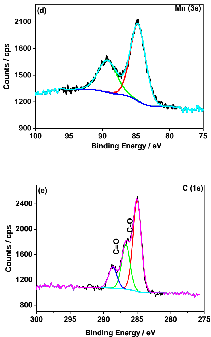
Figure 2 X-ray photoelectron spectroscopy (XPS) spectra (a) wide scan region, (b) Mn 2p , (c) Mn 2p_{3/2} fitting, (d) Mn 3s , and (e) C 1s deconvolution peaks for EMD ( \gamma - \text{MnO}_2 ) samples derived from low-grade residue.
