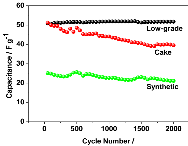
Figure 10 Cycling performance of the activated carbon vs. EMD asymmetric capacitor. EMD derived from different precursors are shown, after 2000 cycles the capacity retention is superior for low grade residue.
