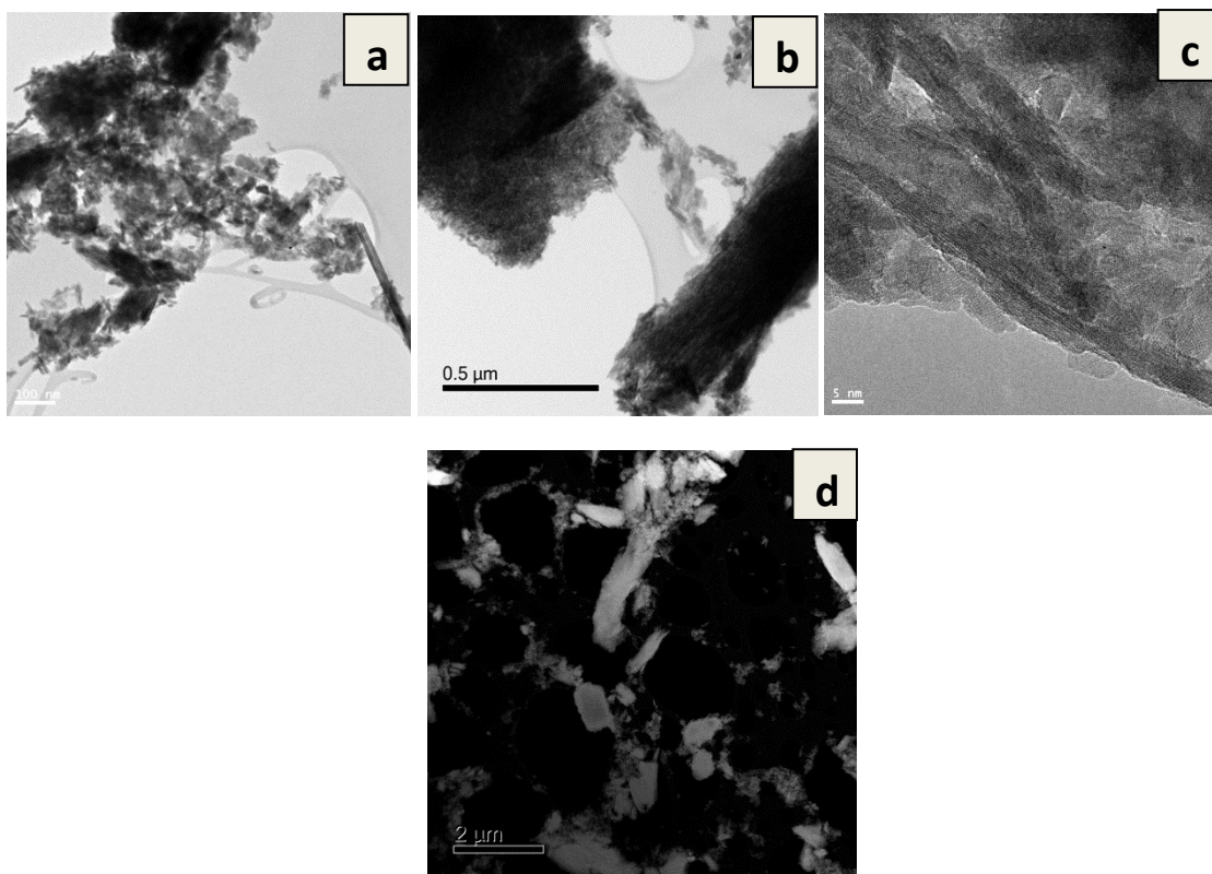
Figure 5 (a) Low magnification bright-field TEM, (b) detailed image of the individual particle showing spindle shape, (c) high resolution TEM (HRTEM) of the spindle shaped particulate and (d) high angle-annular dark field (HAADF) TEM image for EMD ( \gamma - \text{MnO}_2 ) derived from synthetic solution.
