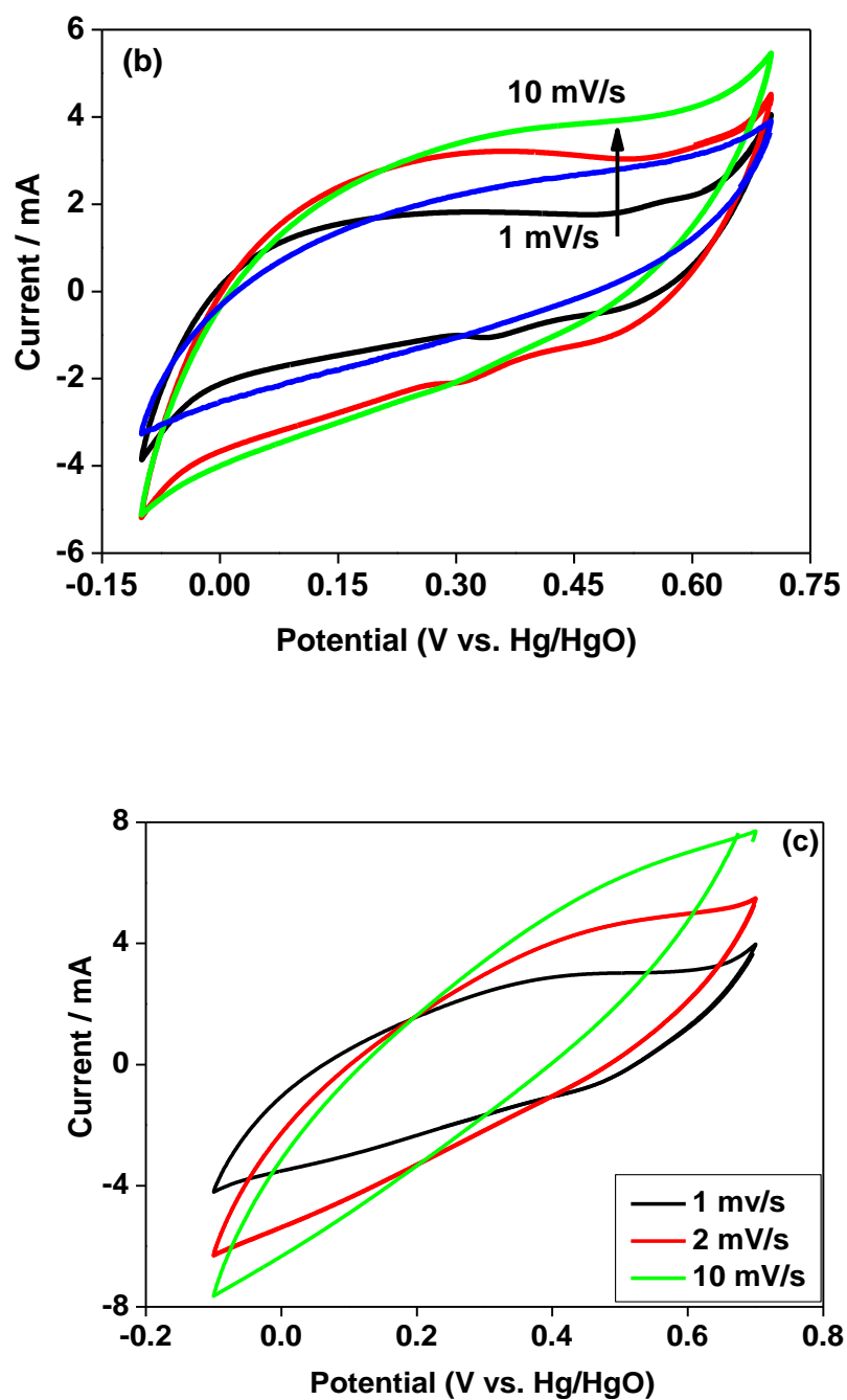
Figure 6 Cyclic voltammogram (CV) measurements of (a) EMD derived from different precursors at 2 mV/s; The effect of scan rate on: b) EMD derived from low-grade residue, and (c) EMD derived from cake. Experiments were performed in a three-electrode system in 2M NaOH electrolyte.
