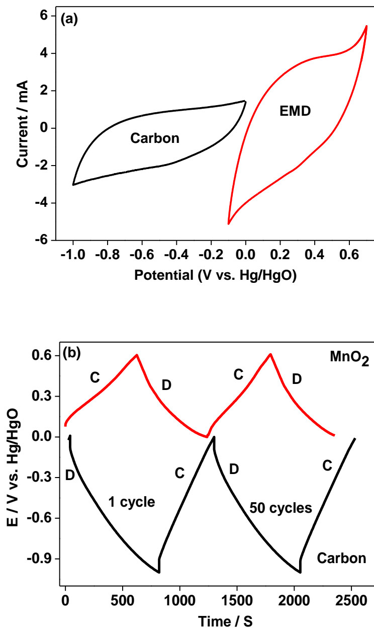
Figure 8 (a) Cyclic voltammogram (CV) curves for activated carbon (AC) negative electrode and EMD positive electrode at 2 mV/s and (b) corresponding galvanostatic (charge-discharge) curves for each electrode at 2 mA. The plots are shown for the 1 st and 50 th cycles. Experiments are performed in a three-electrode system in 2M NaOH electrolyte. (Terms C and D refers to charge and discharge, respectively).
