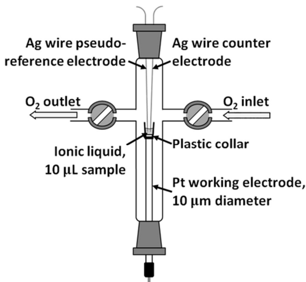
Figure 2. Schematic of the T-cell arrangement used to measure \text{O}_2 electrochemistry in small volumes of IL.
