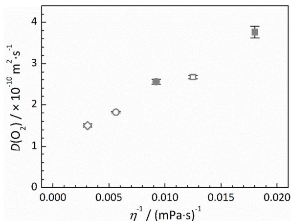
Figure 5. Stokes-Einstein plots for the dependence of the diffusion coefficient of \text{O}_2 , D(\text{O}_2) , on the inverse viscosity, \eta^{-1} , at 297K for [Pyrr 14 ][TFSI] (□), [Pip 14 ][TFSI] (○), [Aze 14 ][TFSI] (◇), [Pyrr 1(2o1) ][TFSI] (■) and [Pip 1(2o1) ][TFSI] (●). The error bars represent the standard error of the measurements.
