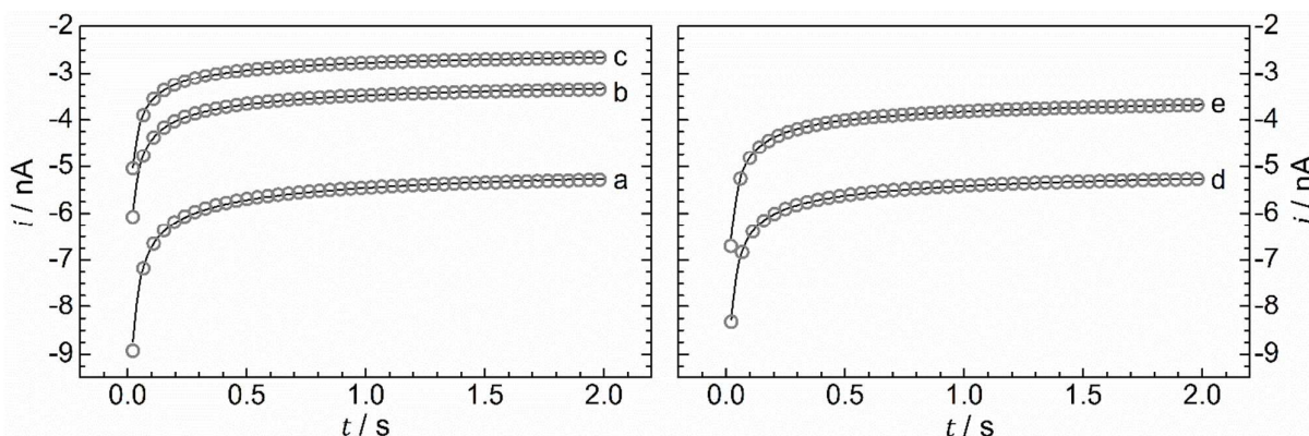
Figure 4. Experimental (—) and simulated (○) chronoamperometric transients for the reduction of \text{O}_2 at 297 \pm 0.5 K under 1 barg \text{O}_2 pressure in (a) [Pyrr 14 ][TFSI] (-1.7 V vs. Ag), (b) [Pip 14 ][TFSI] (-1.75 V vs. Ag), (c) [Aze 14 ][TFSI] (-1.4 V vs. Ag), (d) [Pyrr 1(201) ][TFSI] (-1.88 V vs. Ag) and (e) [Pip 1(201) ][TFSI] (-2.1 V vs. Ag).
