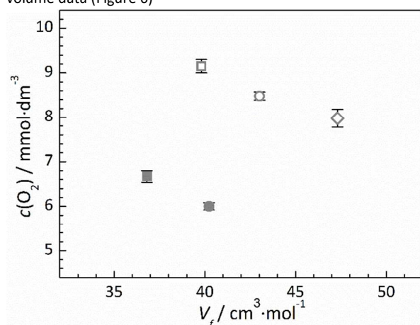
Figure 6. Calculated IL free volume, V_f , versus the solubility of oxygen, c(\text{O}_2) , at 297K for [Pyrr 14 ][TFSI] (□), [Pip 14 ][TFSI] (○), [Aze 14 ][TFSI] (◇), [Pyrr 1(2o1) ][TFSI] (■) and [Pip 1(2o1) ][TFSI] (●). The error bars represent the standard error of the measurements.
