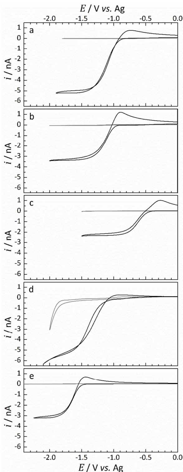
Figure 3. Cyclic voltammograms (black) for the reduction of O_2 at a 10 \mu\text{m} diameter Pt-microdisk electrode vs. Ag in (a) [\text{Pyrr}_{14}][\text{TFSI}] , (b) [\text{Pip}_{14}][\text{TFSI}] , (c) [\text{Aze}_{14}][\text{TFSI}] , (d) [\text{Pyrr}_{1(201)}][\text{TFSI}] and (e) [\text{Pip}_{1(201)}][\text{TFSI}] at 297 \pm 0.5 \text{ K} . The blank traces (grey) were obtained by cyclic voltammetry under an Ar atmosphere prior to exposure to O_2 gas (1 barg). A scan rate of 100 \text{ mV}\cdot\text{s}^{-1} was used in all cases.
