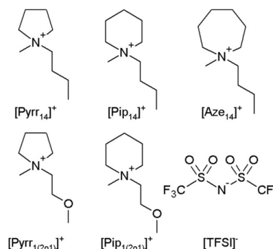
Figure 1. Chemical structures of the cyclic alkylammonium ionic liquid cations and the bis((trifluoromethyl)sulfonyl)imide anion used in this work. The associated abbreviations for each constituent ion are presented.
