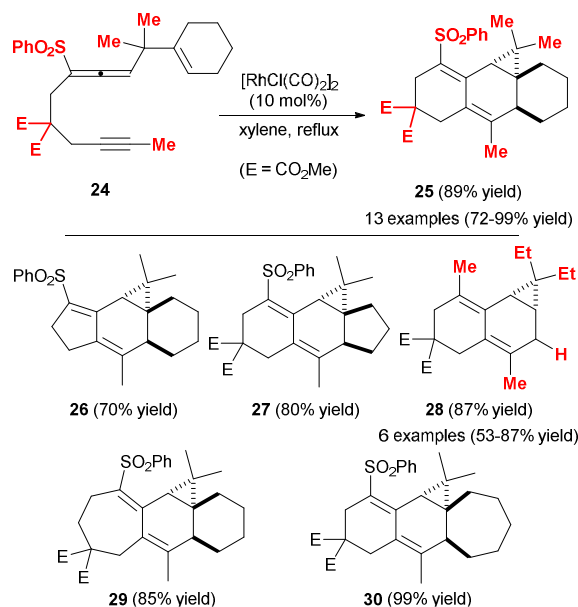
Scheme 10 Rh(I)-catalysed cycloaddition of ene-allene-yne.
