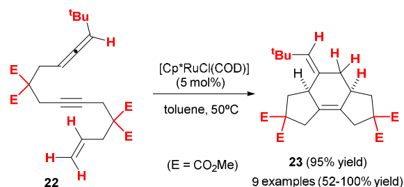
Scheme 9 Ru(II)-catalysed cycloaddition of allene-yne-enes.
