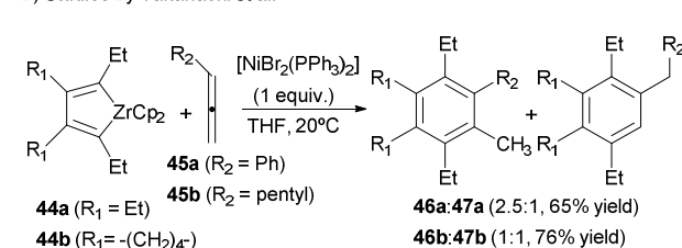
Scheme 14 [2+2+2] Cycloadditions between monoalkynes and diynes with allenes
