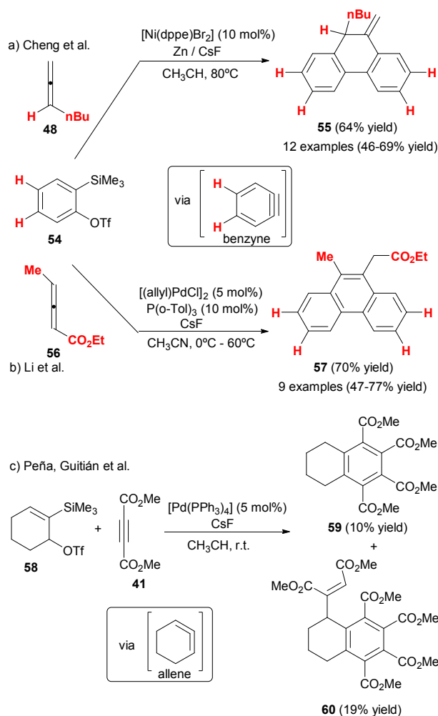
Scheme 16 [2+2+2] cycloadditions involving benzyne and 1,2-cyclohexadienes
