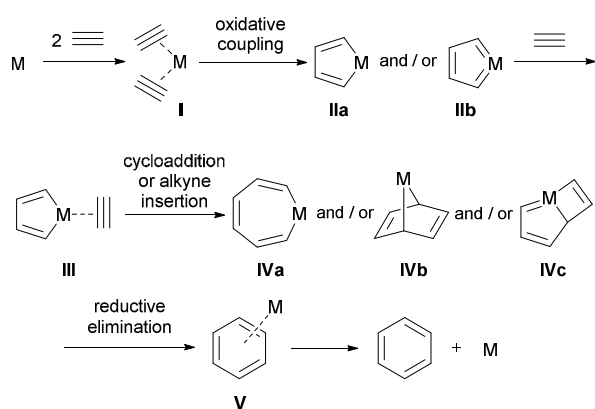
Scheme 2 General overview of the mechanistic cycle of the [2+2+2] cycloaddition reaction of alkynes (M = transition-metal complex).
