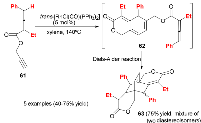
Scheme 17 Rh(I)-catalysed bimolecular cyclisation of propargylic allenoates.
