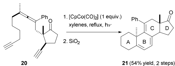
Scheme 8 Diastereoselective synthesis of a steroid-like compound from a diastereomerically pure yne-allene-yne precursor.
