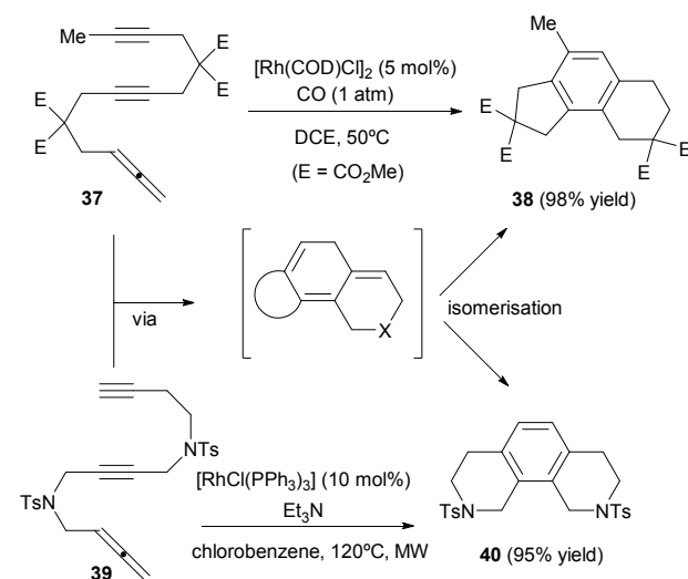
Scheme 13 Rh(I)-catalysed cyclisation/isomerisation of allene-dynes to obtain benzo-fused tricyclic compounds.
