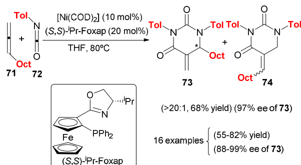
Scheme 20 Ni(0)/( S,S )-Pr-Foxap catalysed enantioselective [2+2+2] cycloadditions between allenes and isocyanates
