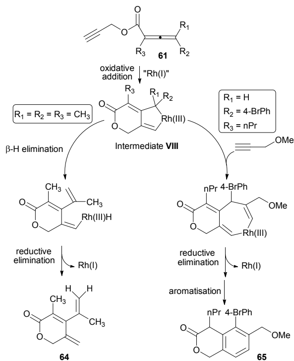
Scheme 18 Mechanistic proposal for the Rh(I)-catalysed unimolecular and bimolecular cyclisations of propargylic allenoates.
